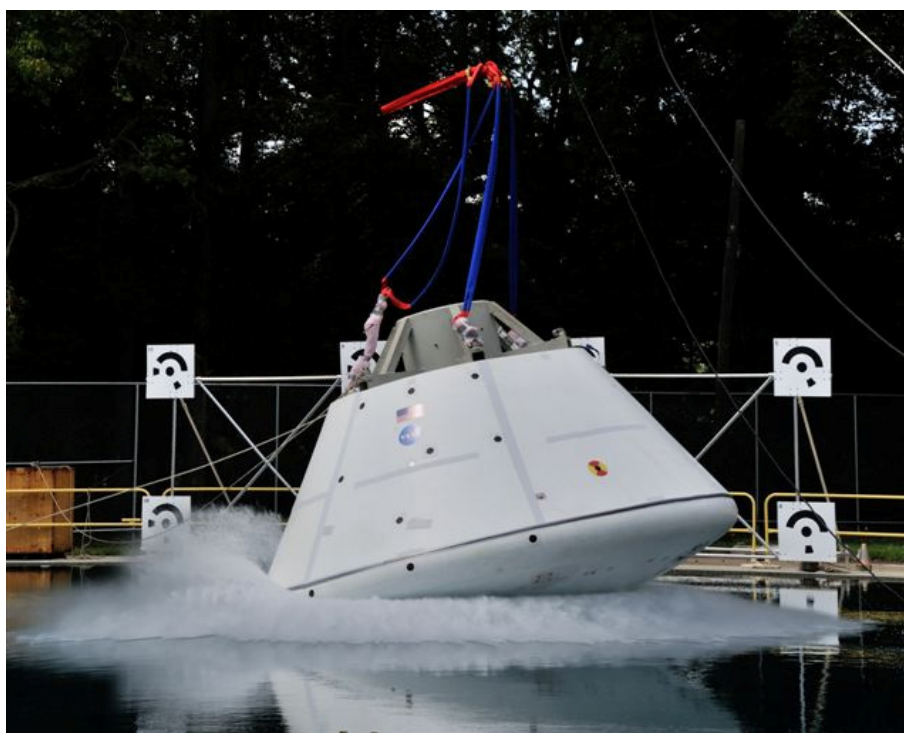
FIGURE 1.7 Water impact test of an 18,000-pound (8,165 kilogram) test version of the Orion spacecraft at NASA's Langley Research Center on August 23, 2012. SOURCE: NASA.
