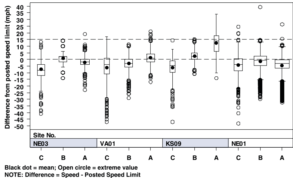
Figure 3-4. Speed differences from posted speed limit—roundabouts.
