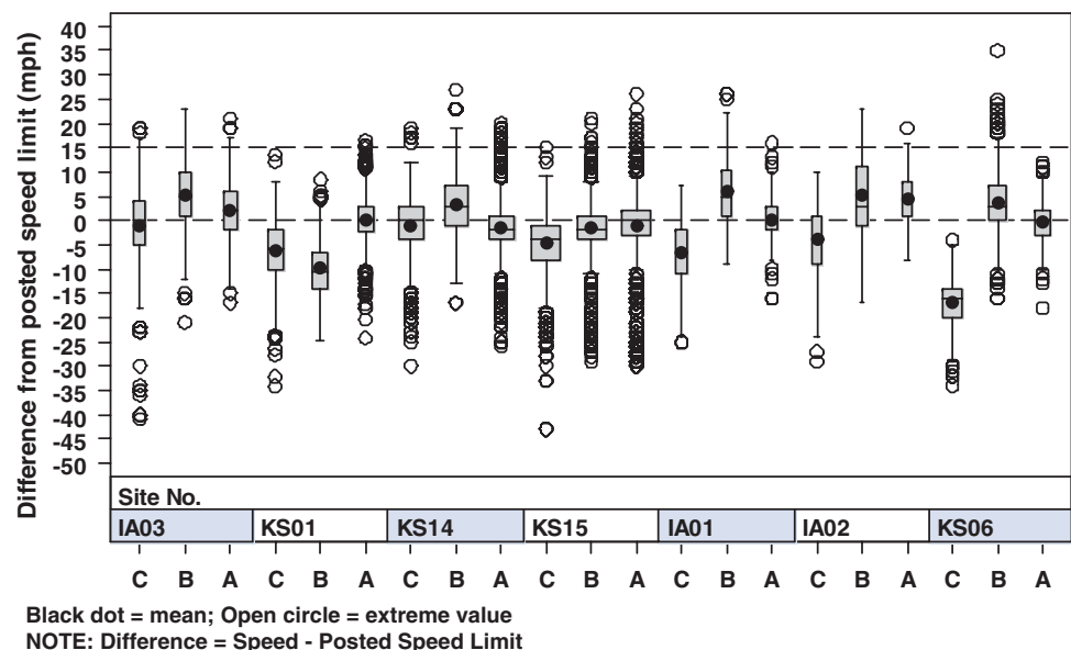
Figure 3-5. Speed differences from posted speed limit—TPMs.
