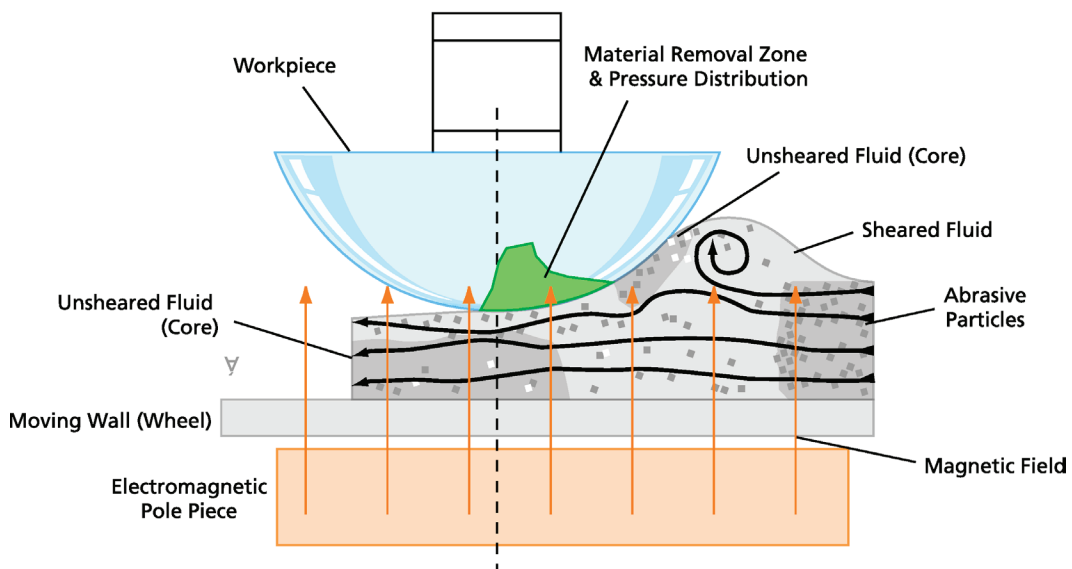
FIGURE C.12 Magnetorheological finishing polishing. SOURCE: Reprinted with permission from Photonics Tech Briefs .
