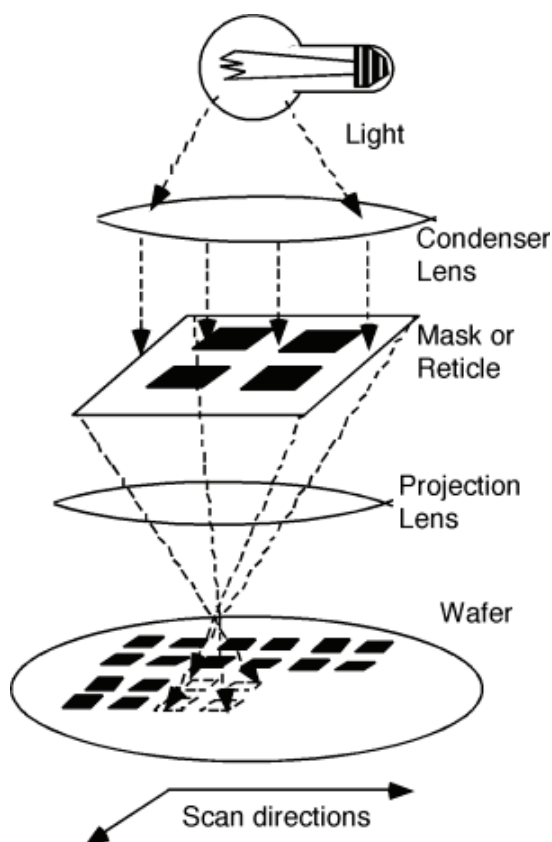
FIGURE 7.7 Generic schematic diagram of the lithographic process. SOURCE: Bill Wilson. 2007. "Photolithography." Connexions . Available at http://cnx.org/content/m1037/2.10/ . Reprinted with permission.
