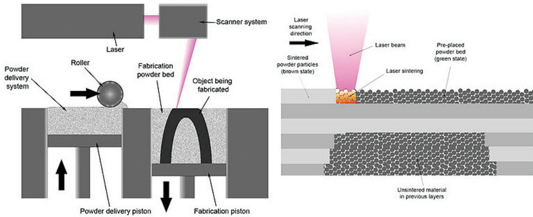
FIGURE 7.13 Selective laser sintering (SLS) schematic. SOURCE: Image by Materialgeeza.
