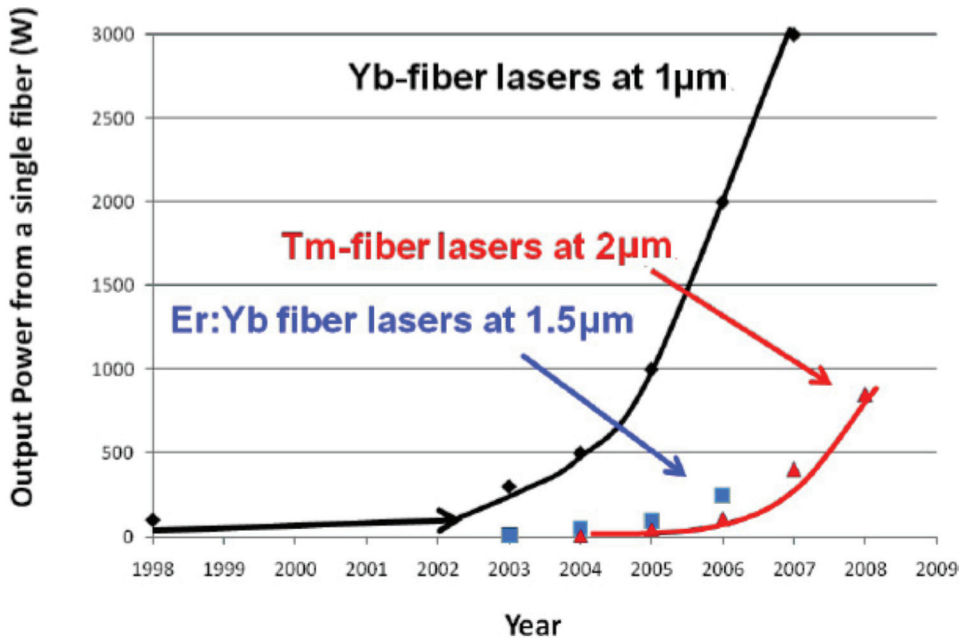
FIGURE C.1 Progress in output power for 1 \mu m, 1.5 \mu m, and 2 \mu m optical amplifiers. This plot tracks the historical progress in output power from a single fiber amplifier. Ytterbium (Yb)-fiber amplifiers (1 \mu m) have a significant lead over other technologies primarily due to their low quantum defect and the abundance of high-brightness pump sources at 915 to 975 nm. However, thulium (Tm)-fiber amplifiers (1.9 to 2.1 \mu m) have been demonstrated with average output powers approaching 1 kW and pulsed operation approaching 100 kW without sacrificing beam quality. There are several commercial units available with an average power \sim 150 W. Their efficiency is set by the efficiency of the pump source, which should continue to improve over time as demand for Tm-lasers increases. SOURCE: Cristensen, S., G. Frith, and B. Samson. 2008. "Developments in Thulium-Doped Fiber Lasers Offer Higher Powers." SPIE Newsroom . DOI: 10.1117/2.1200807.1152. Available at http://spie.org/x26003.xml . Reprinted with permission.
