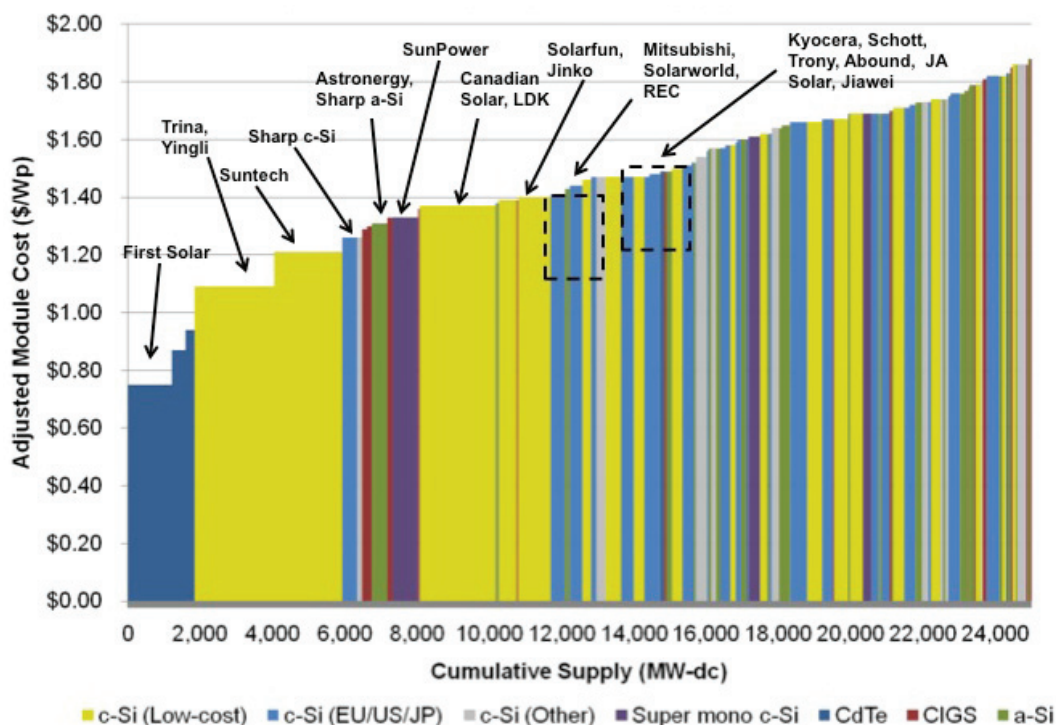
FIGURE 5.3 Average cost per watt of current widely deployed photovoltaic technologies in 2011. SOURCE: "PV Technology, Production and Cost Outlook: 2010-2015" (GTM Research). Reprinted with permission.
