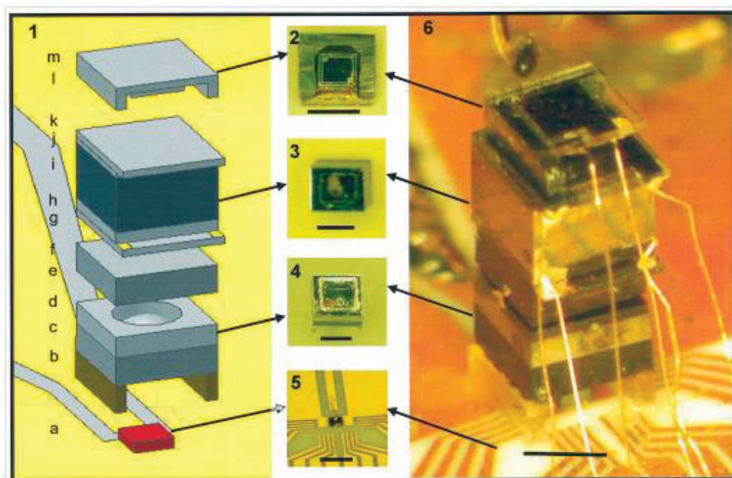
FIGURE 8.1 Schematic ( left ) and photograph ( right ) of a microfabricated atomic clock. The total volume of the device is less than 1 \text{ cm}^3 , making it practical for use in handheld, battery-powered electronics. (See source for detailed image labels.) SOURCE: Reprinted, with permission, from Knappe, S., L. Liew, V. Shah, P. Schwindt, J. Moreland, L. Hollberg, and J. Kitching. 2004. A microfabricated atomic clock. Applied Physics Letters 85:1460.
