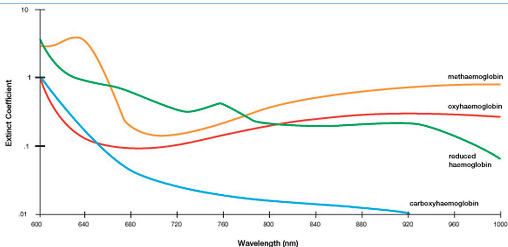
FIGURE C.7 Blood changes color depending on the hemoglobin status. The absorption profiles of four different hemoglobin statuses are shown. Simple disposable probes that can be mounted on a patient's finger can precisely measure the absorption level of the blood at different wavelengths and help determine the extent and cause of hypoxia. SOURCE: Masimo. 2012. "Rainbow SET Pulse CO-Oximetry." Available at http://www.masimo.co.uk/Rainbow/about.htm . Reprinted with permission.
