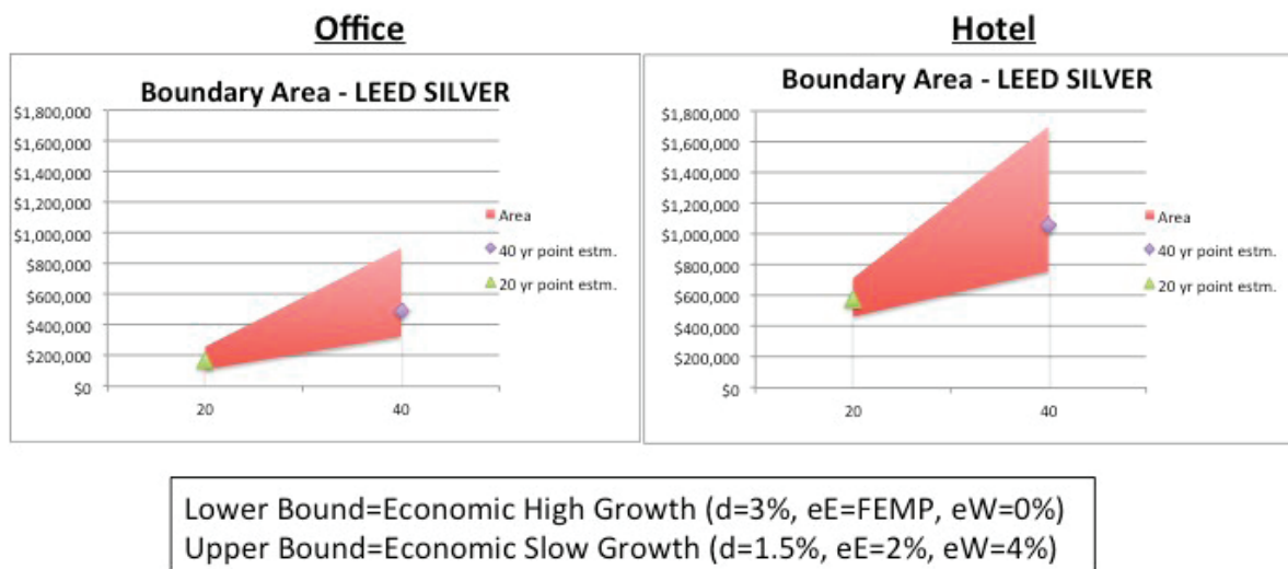
Figure 18: LEED Sensitivity Analysis for Net Savings: Phoenix
