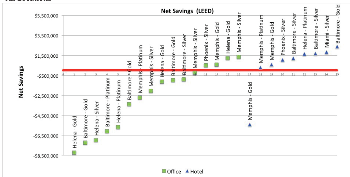
Figure 16: LEED Long-term Cost-Benefit: Net Savings for All Buildings, All Certification Levels, and All Locations
