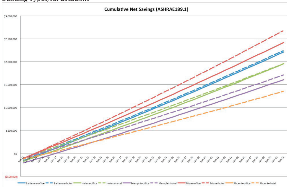
Figure 15: ASHRAE 189.1-2011 Simple Payback through Cumulative Annual Net Savings: All Building Types, All Locations
