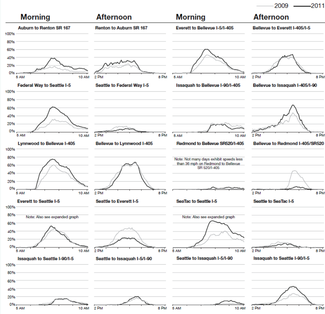
Figure 2.6. Washington State DOT’s tracking of travel times in general purpose (GP) lanes (4).
