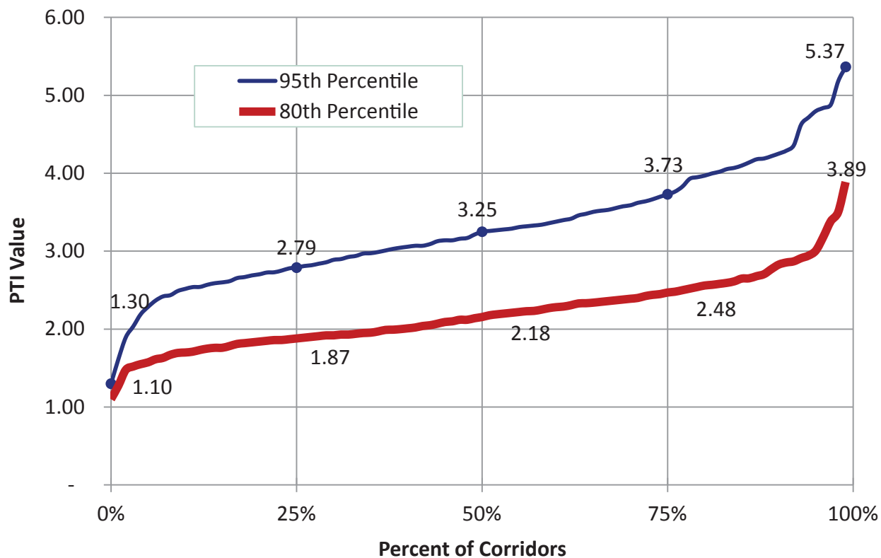
Figure 4.2. Distribution of the PTI for the 328 most congested corridors in the United States (2).
