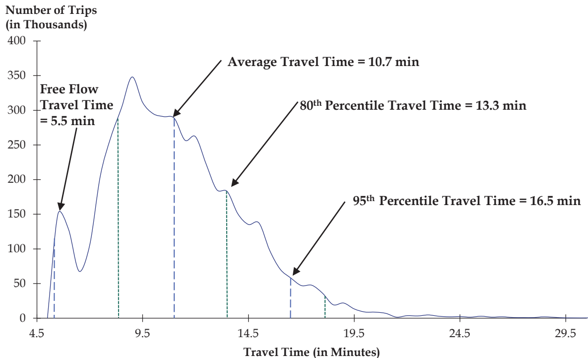
Figure ES.1. Distribution of travel times for a single roadway segment.
