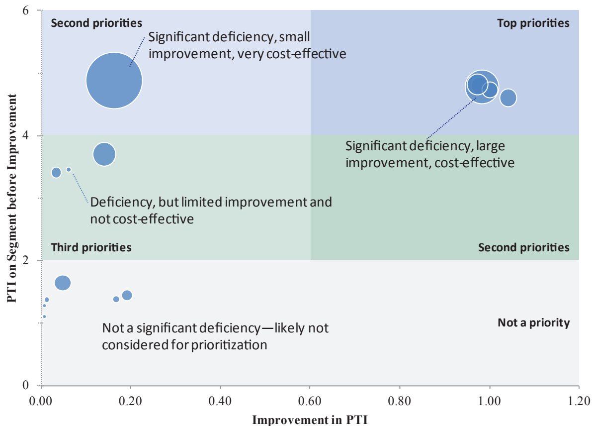
Figure 5.4. Example prioritization scheme of Knoxville operations and management investments. Note that bubbles are sized relative to the cost-effectiveness of the proposed projects.
