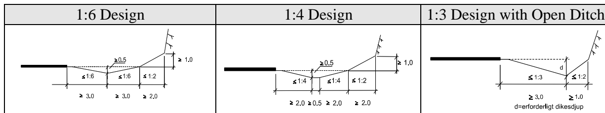
FIGURE 2 Verge designs.
