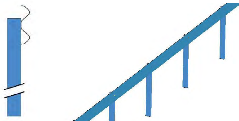
FIGURE 2 AG04-2.0: (a) guardrail components and (b) finite element model (4).
