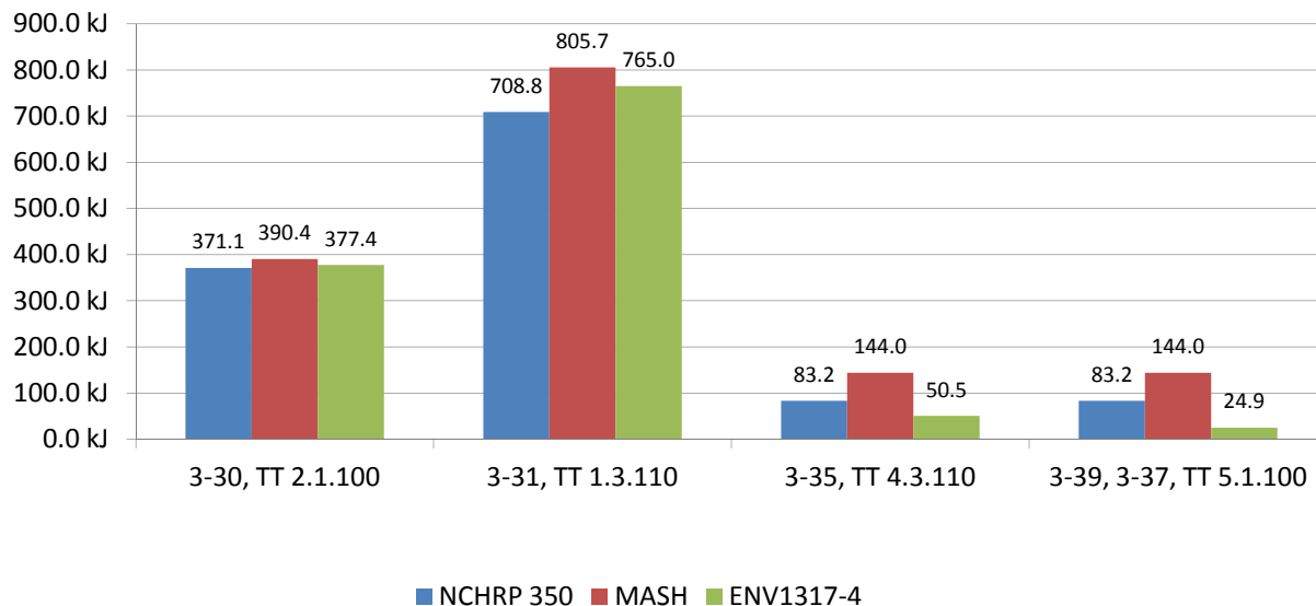
FIGURE 6 Adjusted KE to tolerances for redirective end terminals for NCHRP 350, MASH, and ENV 1317-4.
