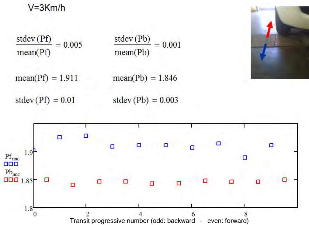
FIGURE 5 Results of test at slow speed (3 km/h) with back-and-forth transit of front wheel on the WIM bending plate: Pf, forward, blue data; Pb, backward, red data. Weight values are given in arbitrary units. Results show evidence of different weight measurement for the dynamic load of the front wheel (picture, right) transiting forward and backward, as expected from shock absorber with acc \neq 0 motion.
