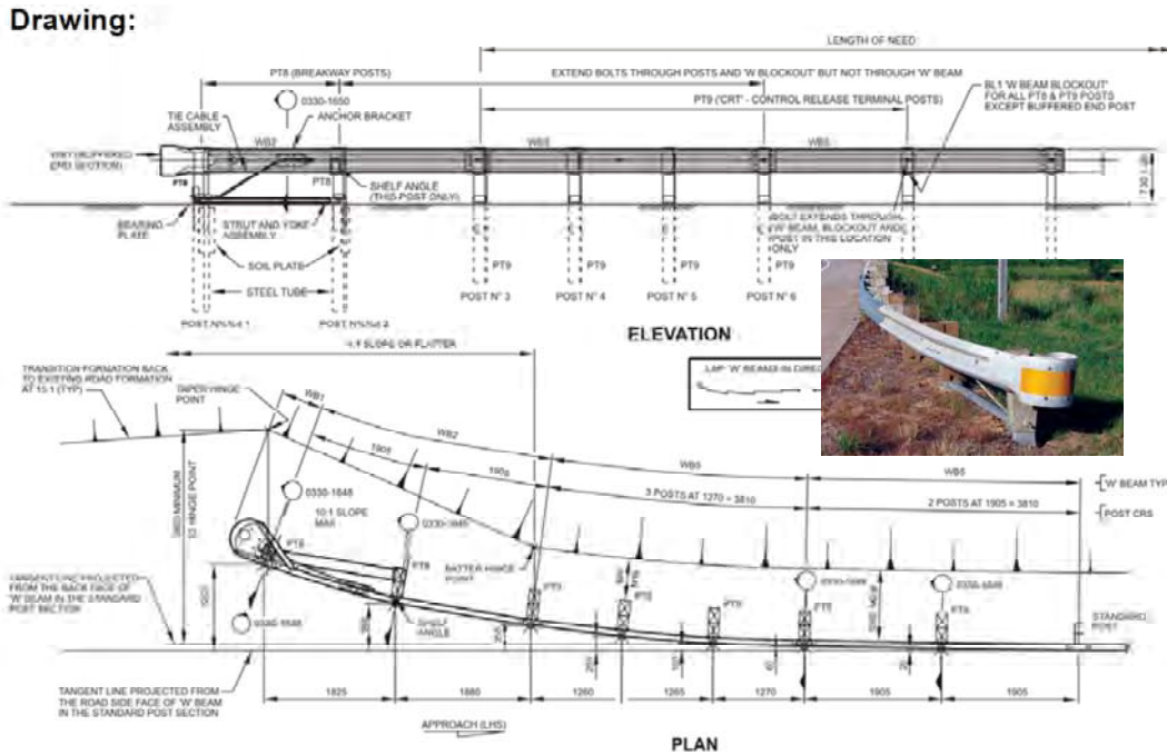
FIGURE 3 Nonpatented crashworthy barrier terminal. [From Main Roads Washington, website with photo from AASHTO (2011).]
