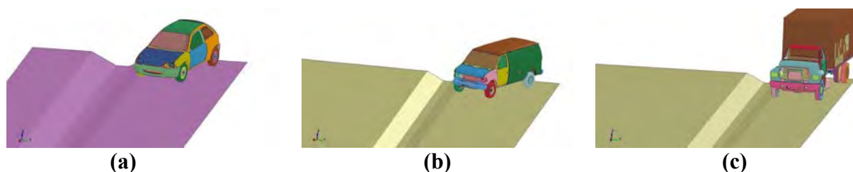
FIGURE 3 Finite element model of ditch and vehicles used in the simulations: (a) 900-kg automobile, (b) 3,000-kg van, and (c) 10,000-kg truck.
