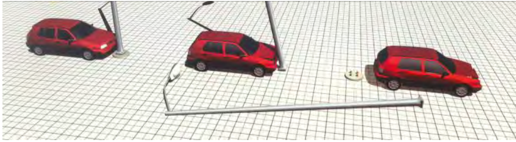
FIGURE 1 Breakaway pole collapse mechanism.
