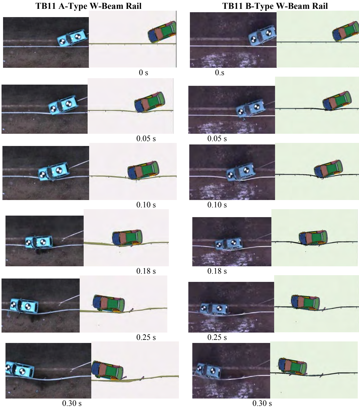
FIGURE 3 TBLL crash test and LS-DYNA simulation comparison for AG04-2.0 guardrail.
