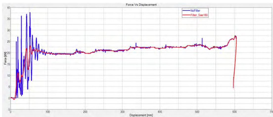
FIGURE 2 Force versus displacement curve for the steel honeycomb energy absorber. Blue curve: data from the calculation; red curve: SAE 180 filtered curve.
