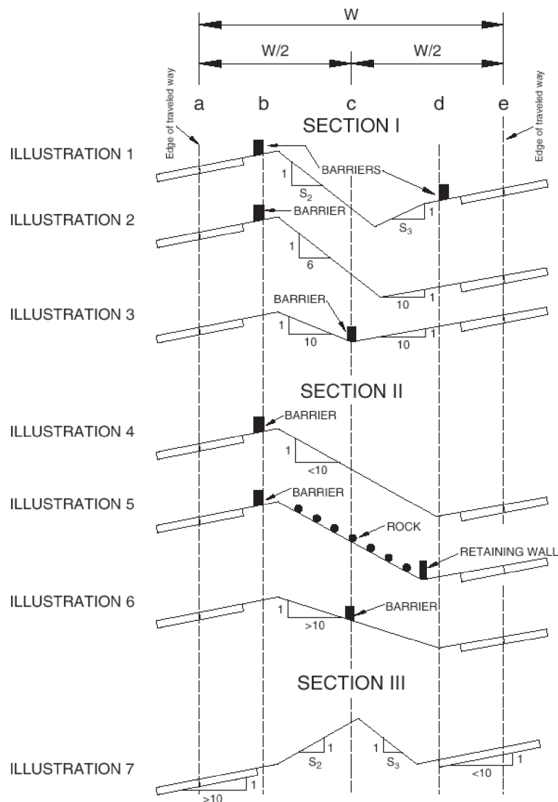
Figure 2-3. Median barrier placement guidelines (2).
