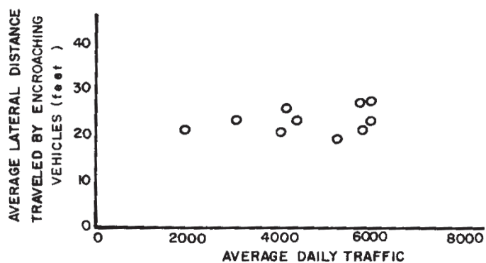
Figure 2-7. Relationship between ADT and encroachment distance (4).
