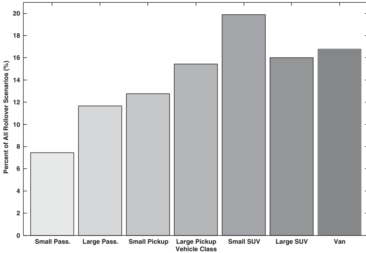
Figure 5-3. Rollover scenarios for all vehicle classes.
