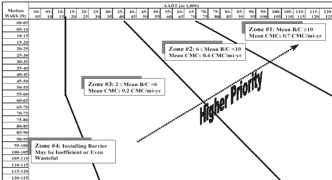
Figure 2-9. Benefit-cost ratios based on Texas study (16).
