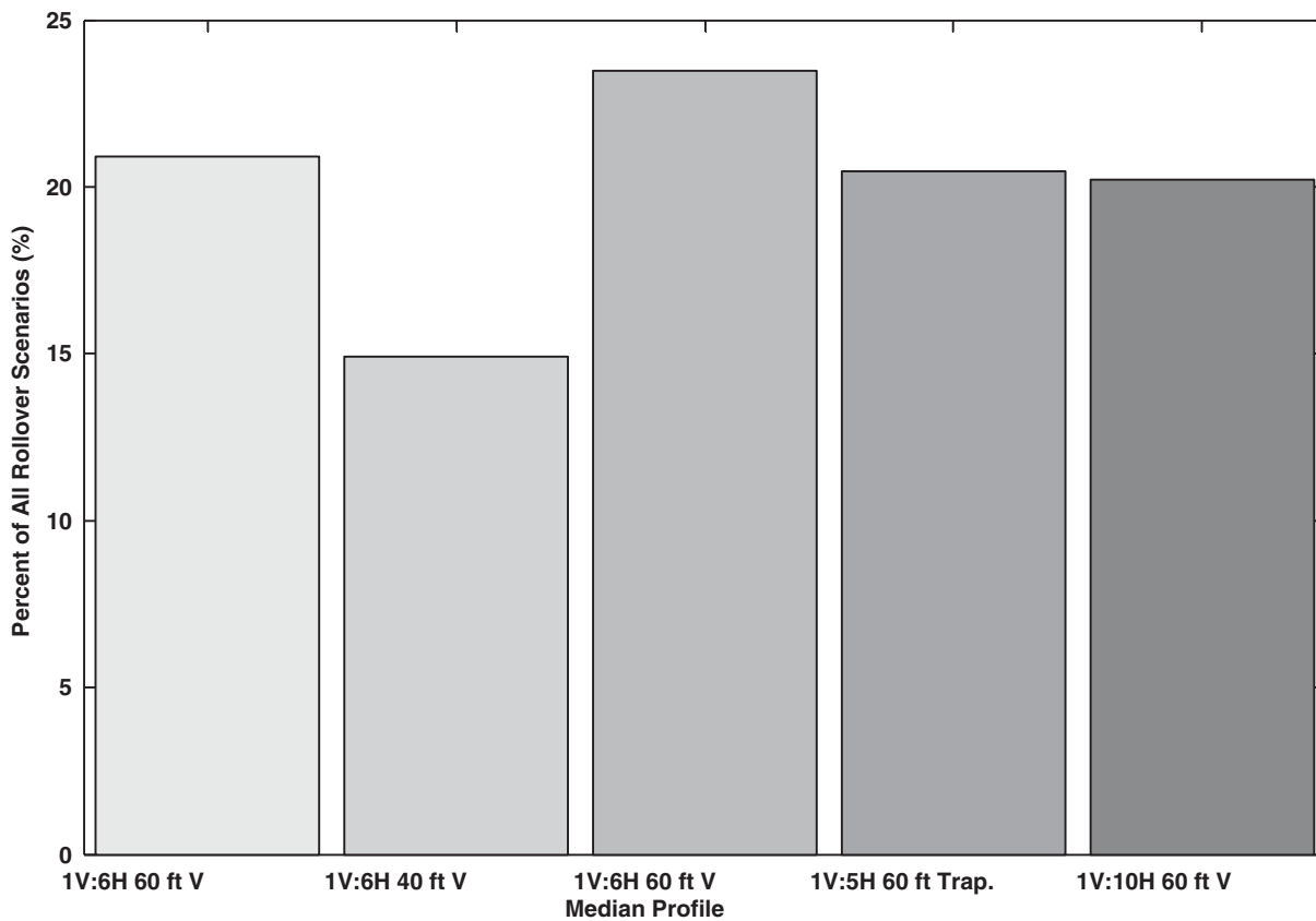
Figure 5-4. Effect of median profile on vehicle rollover.
