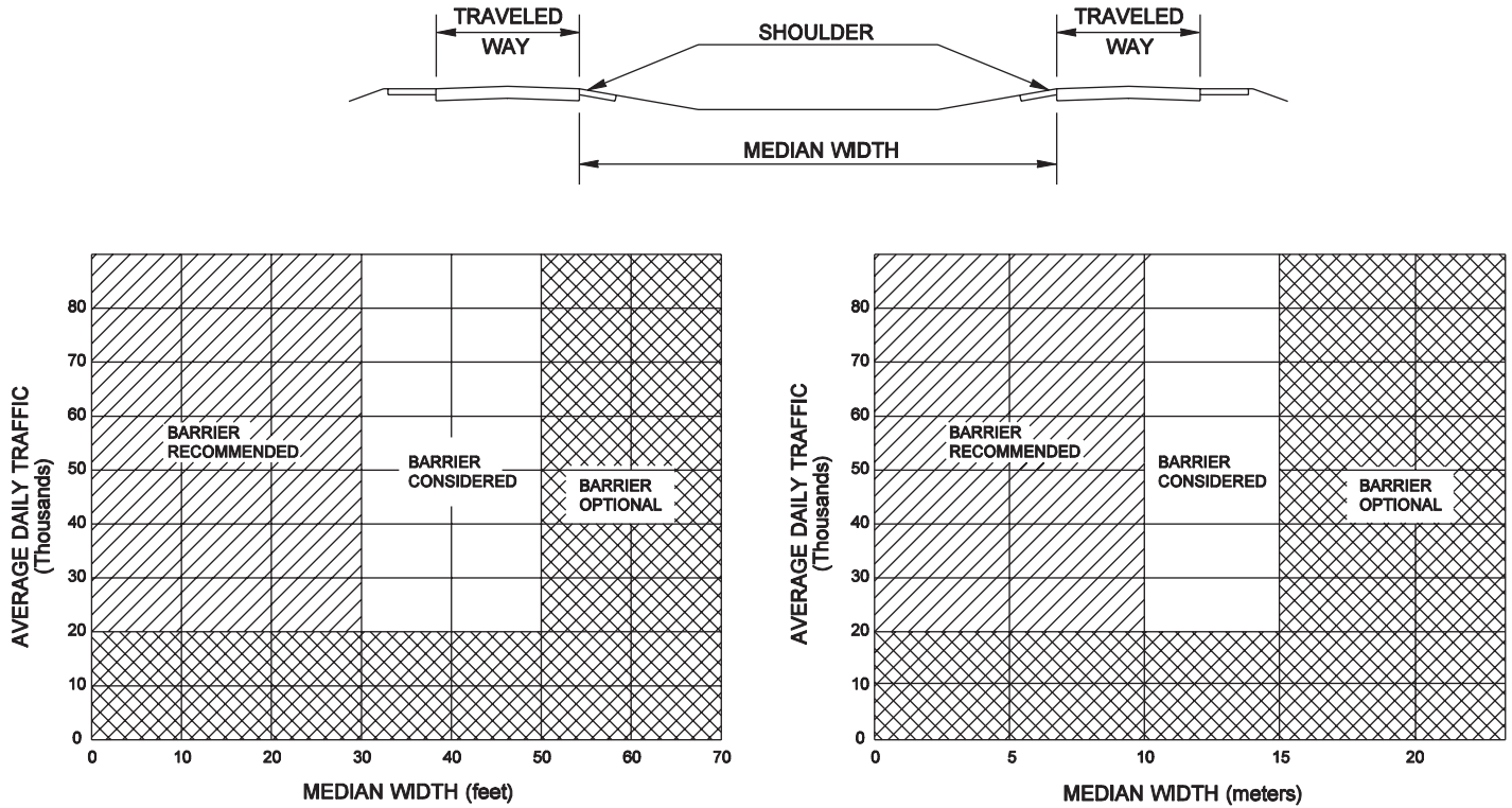
Figure 2-2. Guidelines for median barriers on high-speed, fully controlled-access roadways from 2006 AASHTO Roadside Design Guide (2).
