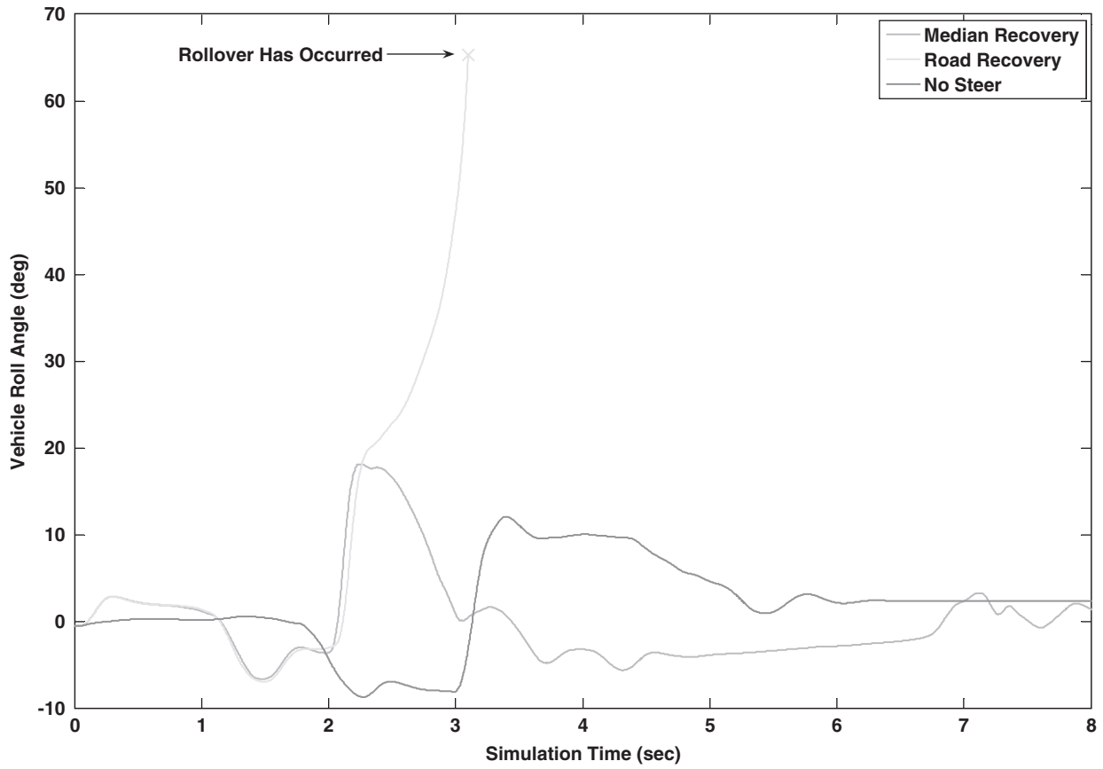
Figure 5-20. Roll angle for varied steering input.
