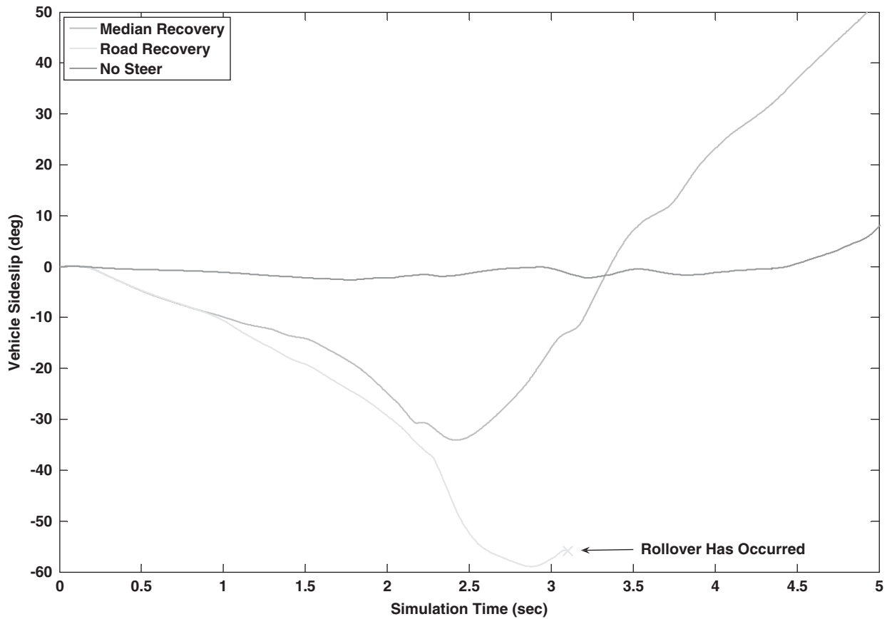
Figure 5-21. Sideslip for varied steering input.
