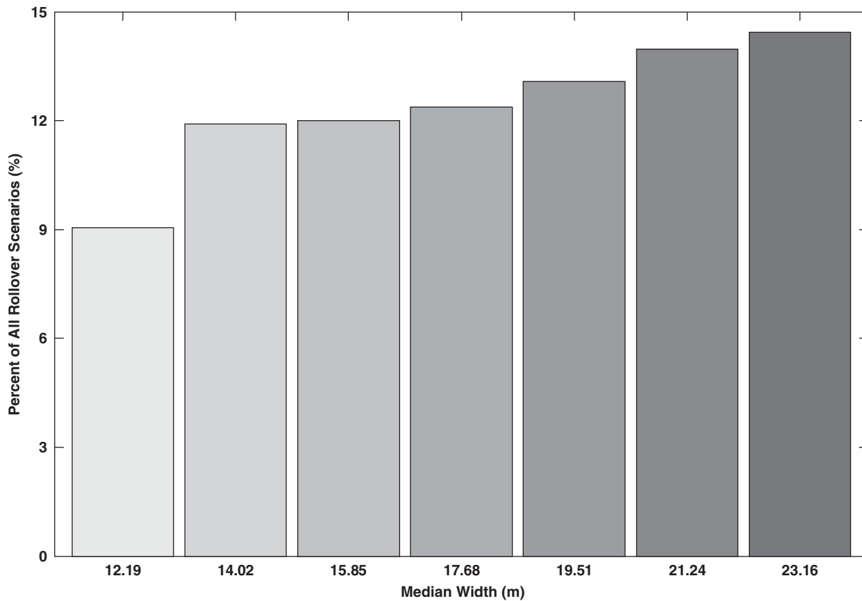
Figure 5-10. Effect of median width on vehicle rollover.
