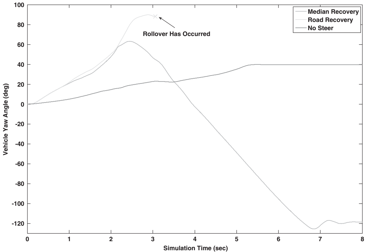
Figure 5-19. Yaw angle for varied steering input.
