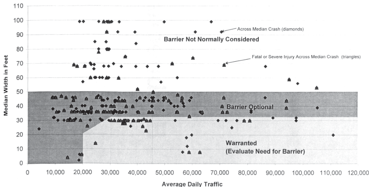
Figure 2-10. Cross-median crashes on North Carolina divided freeways (18).
