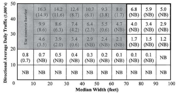
(b) W-Beam Guiderail Median Barrier
