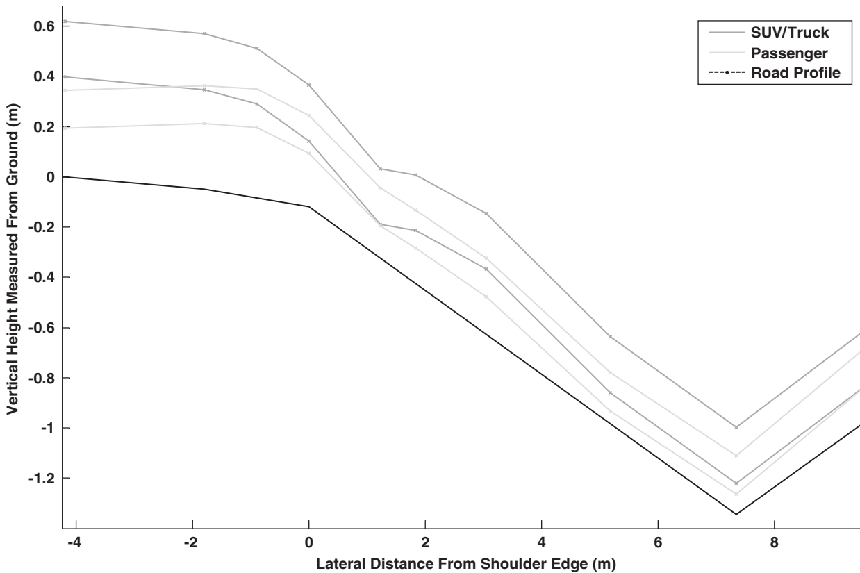
Figure 5-25. Bumper height and clearance modes throughout the median incursion.
