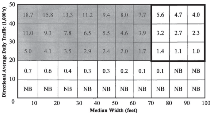
(a) Concrete Median Barrier
