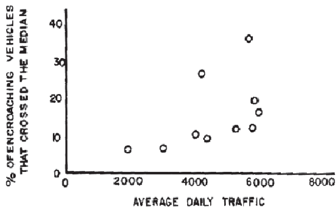
Figure 2-6. Relationship between ADT and percent vehicles crossing into median (4).
