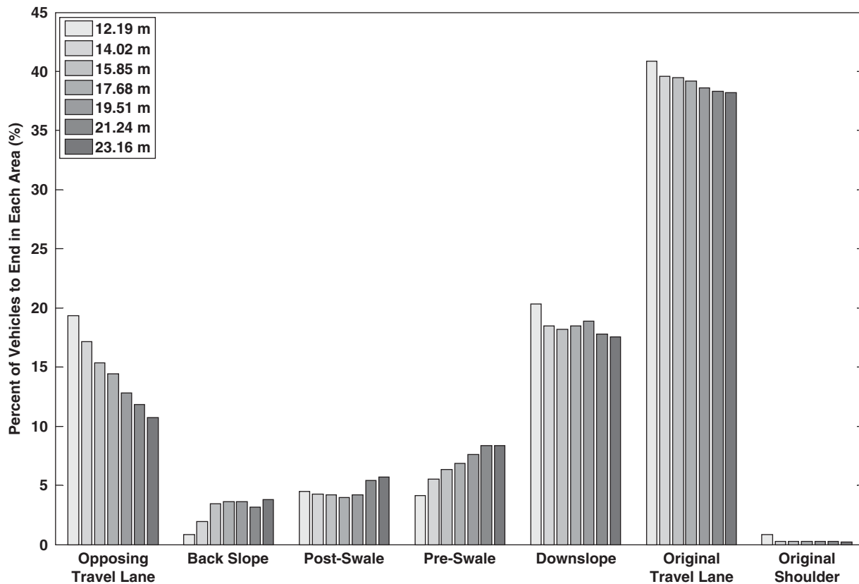
Figure 5-11. End locations for non-rollover simulation runs for medians of varied width.
