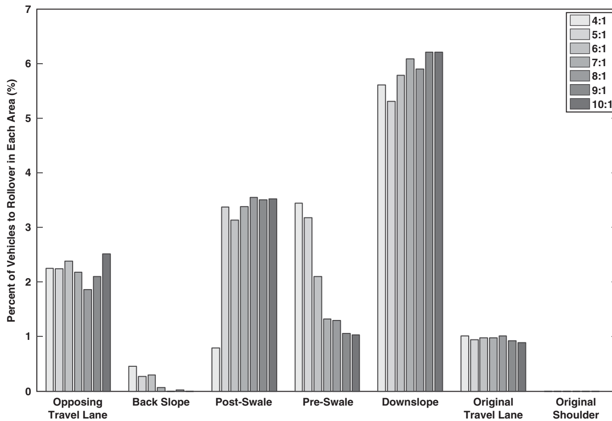
Figure 5-7. Vehicle locations at the onset of rollover for medians of varied slope.
