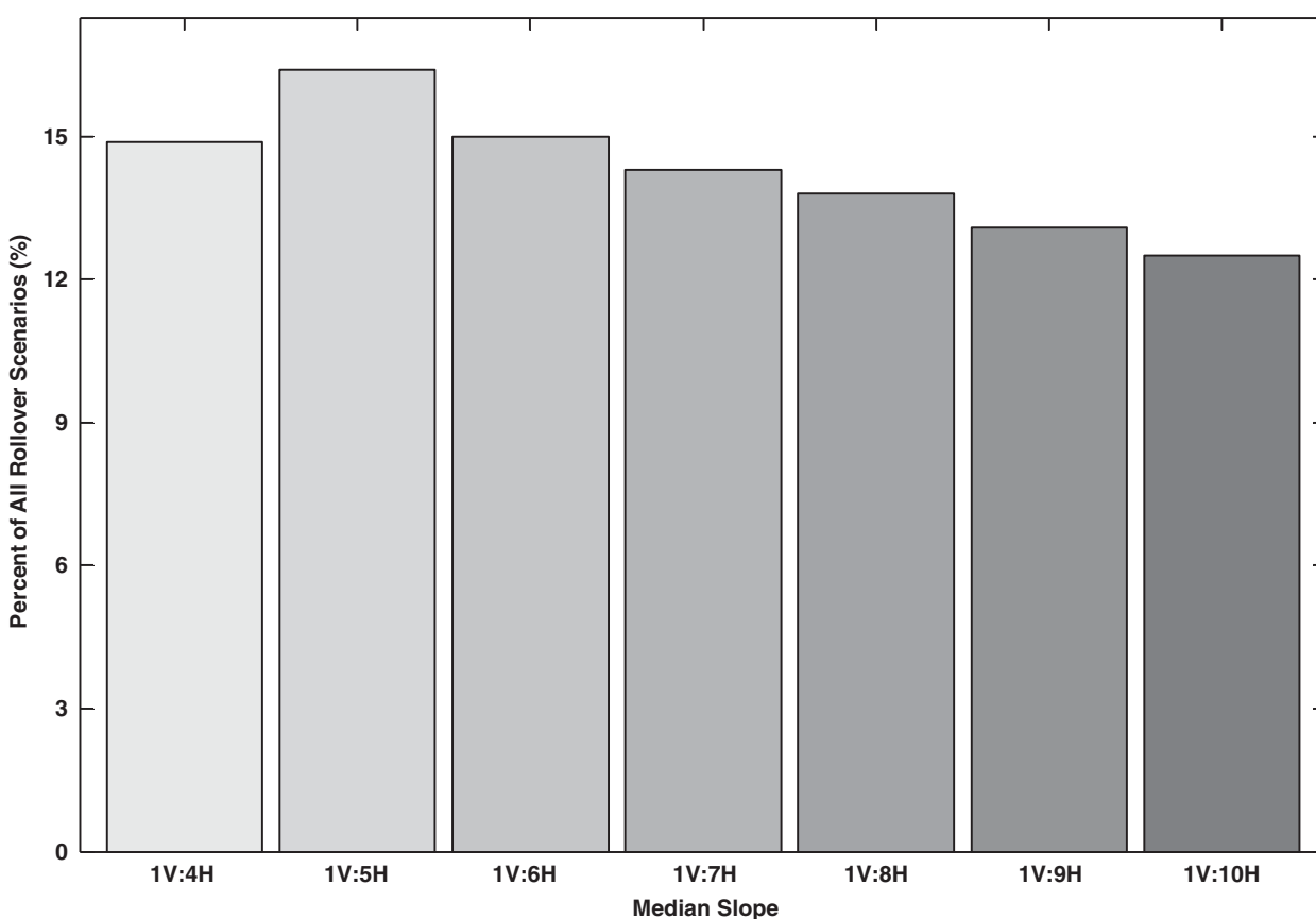
Figure 5-5. Effect of median slope on vehicle rollover.
