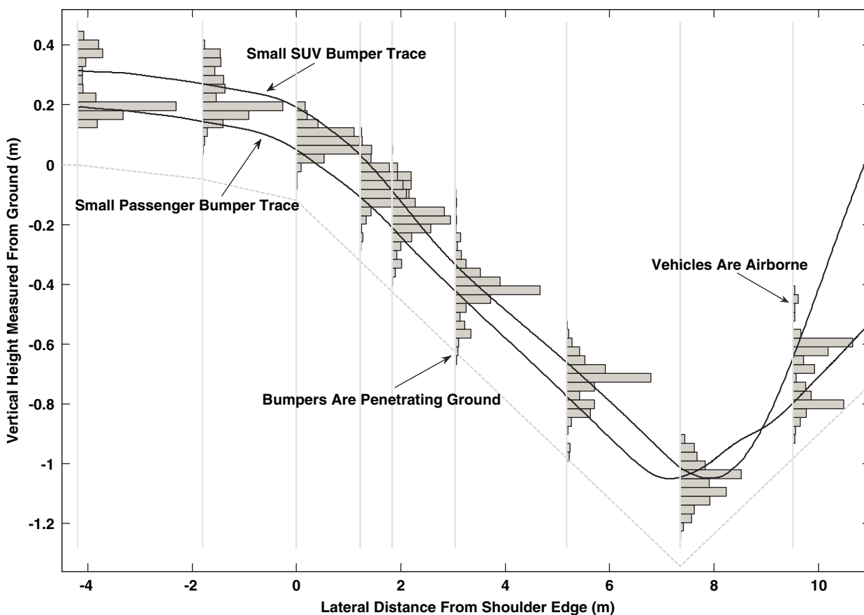
Figure 5-15. Bumper height distributions at various lateral offsets from shoulder edge.
