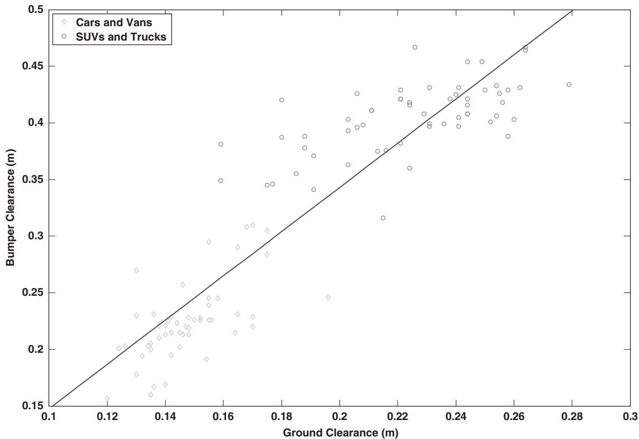
Figure 5-13. Inferring initial bumper height.
