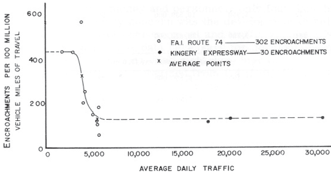
Figure 2-4. Encroachment rate for Interstate 74 and Kingery Expressway (4).
