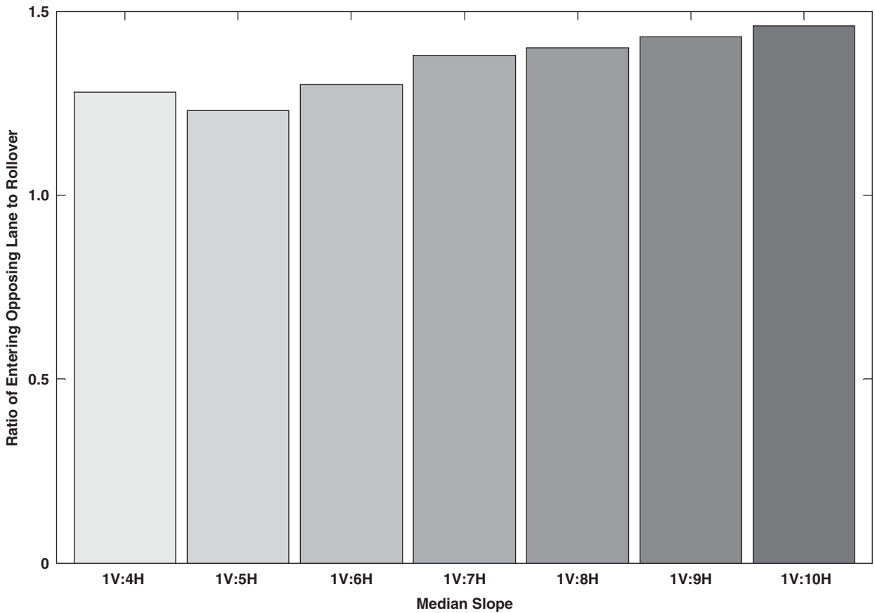
Figure 5-9. Ratio of vehicles entering opposing lane to rollover for medians of varied slope.
