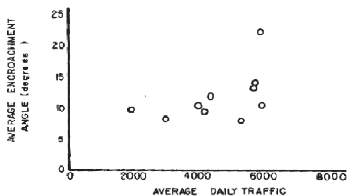
Figure 2-5. Relationship between ADT and average encroachment angle (4).
