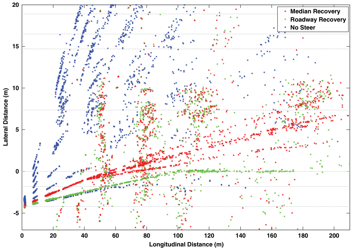
Figure 5-22. Final vehicle position.
