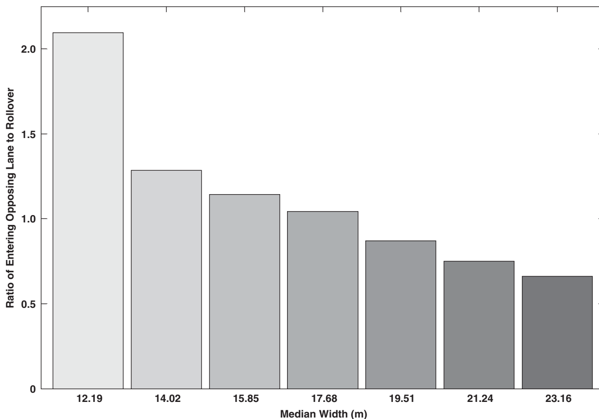
Figure 5-12. Effect of median width on vehicle response.
