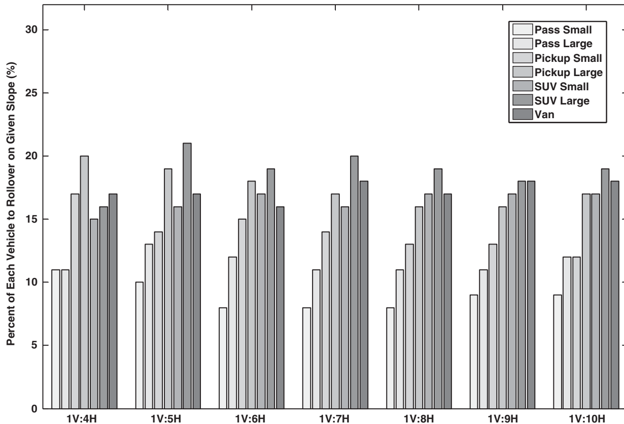
Figure 5-6. Rollover in medians of varied slope by vehicle class.
