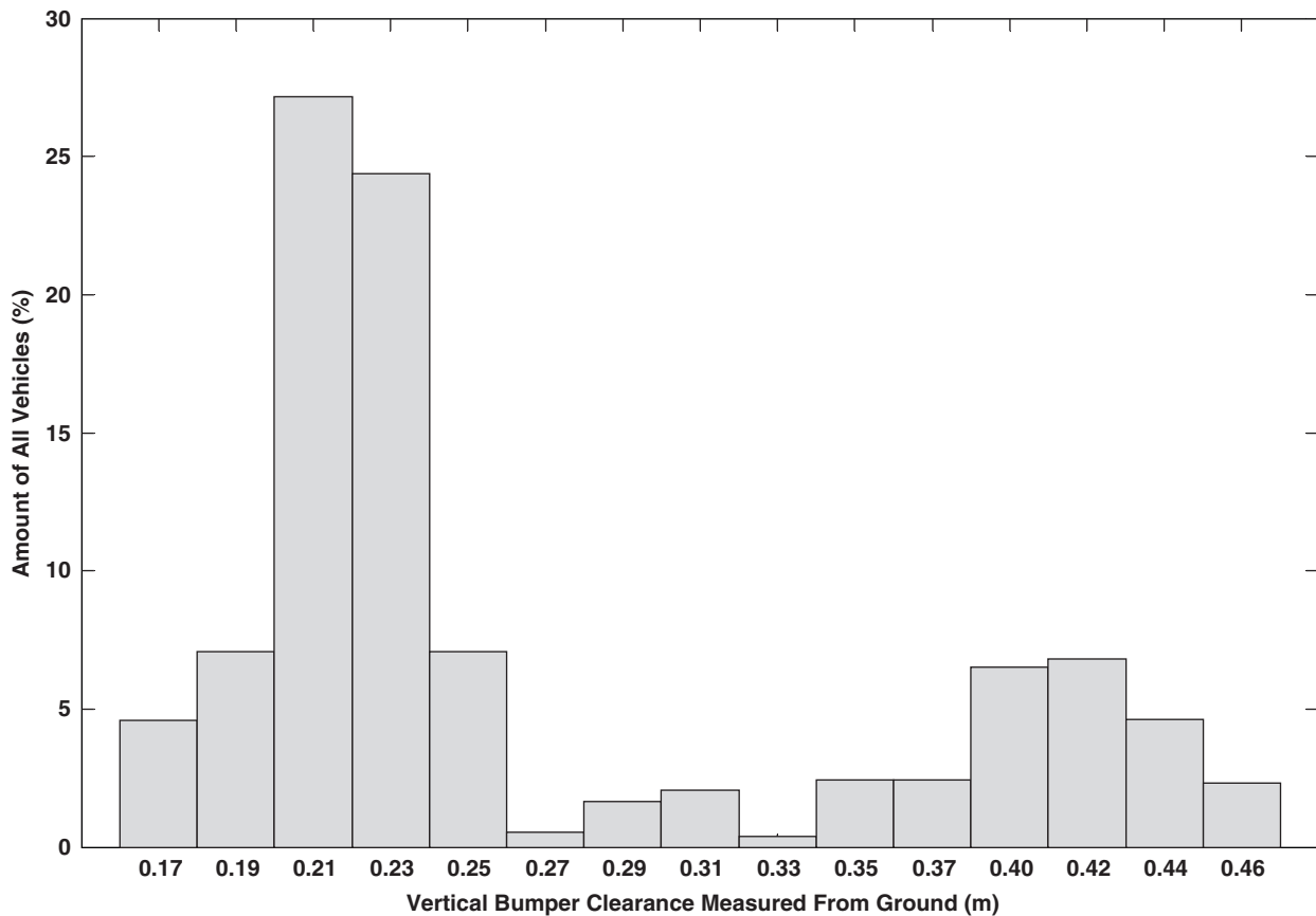
Figure 5-14. Initial bumper clearance distribution.
