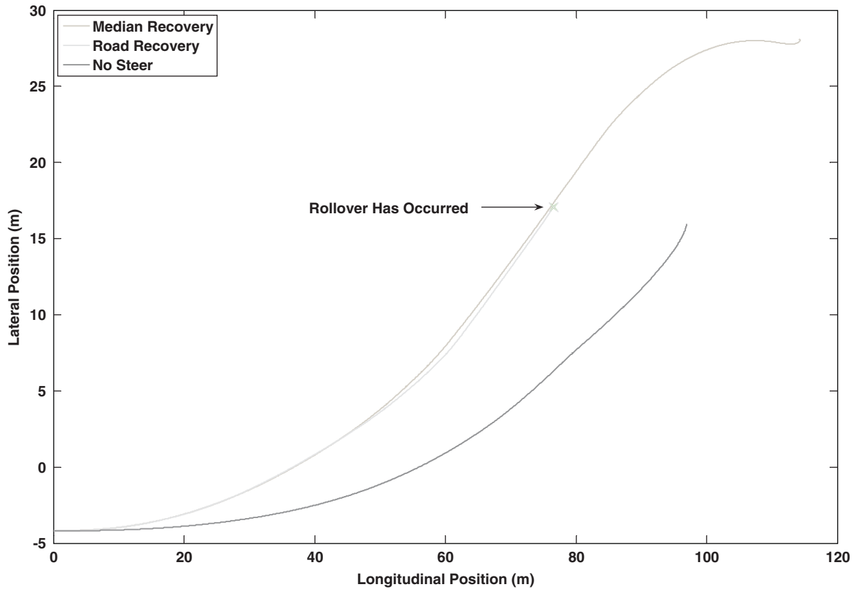
Figure 5-18. XY position for varied steering input.
