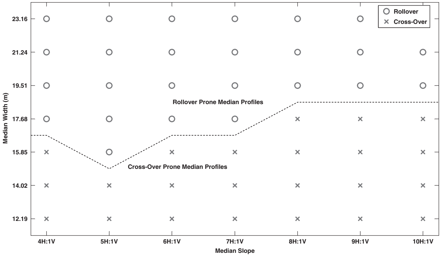
Figure 5-24. Optimal median geometry analysis.
