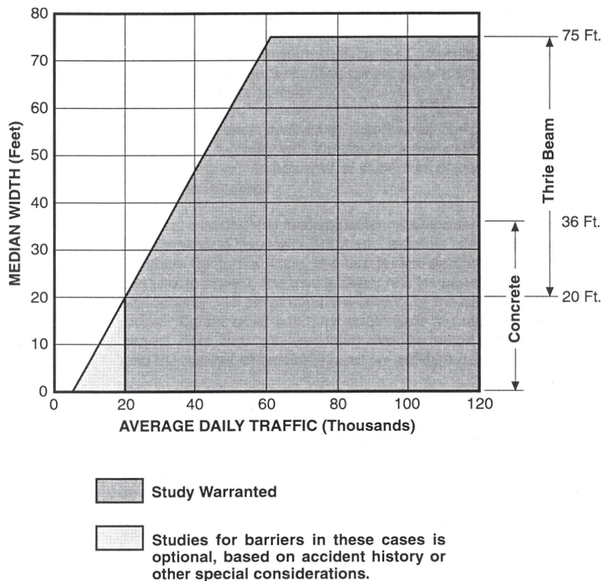
Figure 2-11. California freeway median barrier warrant (19).
