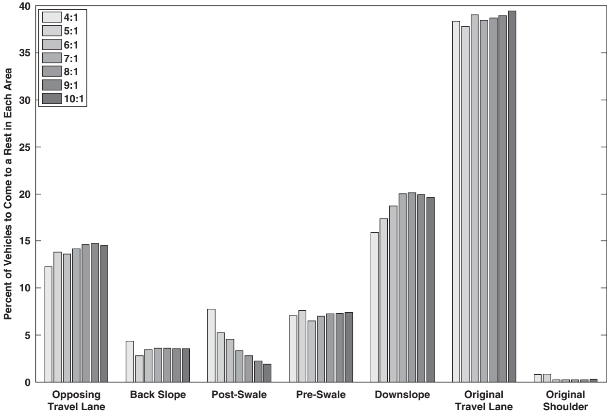
Figure 5-8. End locations for non-rollover simulation runs for medians of varied slope.
