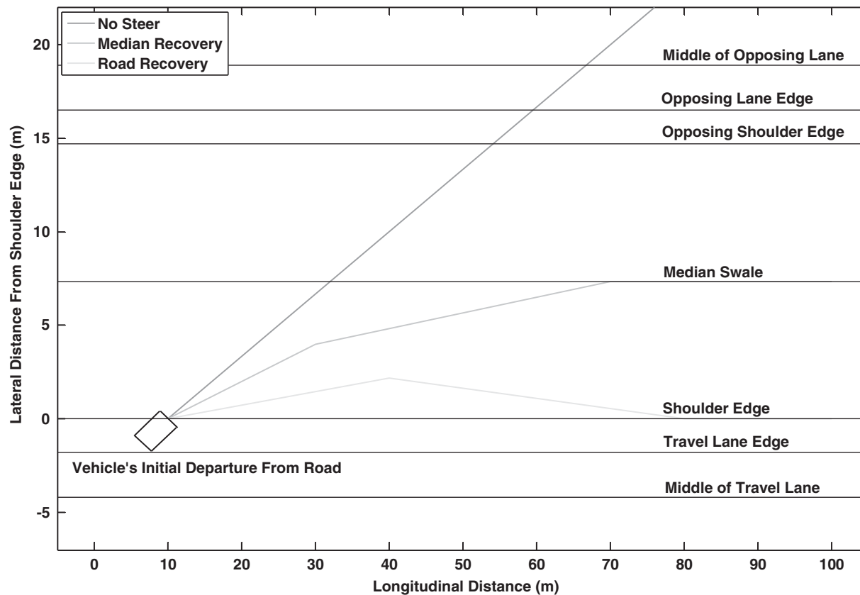
Figure 5-2. Steering inputs used in simulations.
