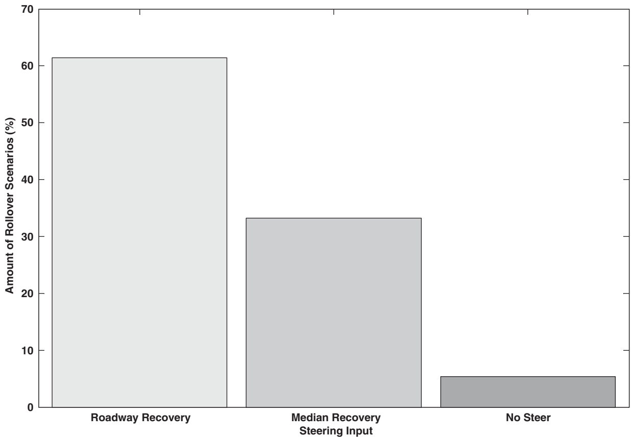
Figure 5-23. Effect of steering input on vehicle rollover.
