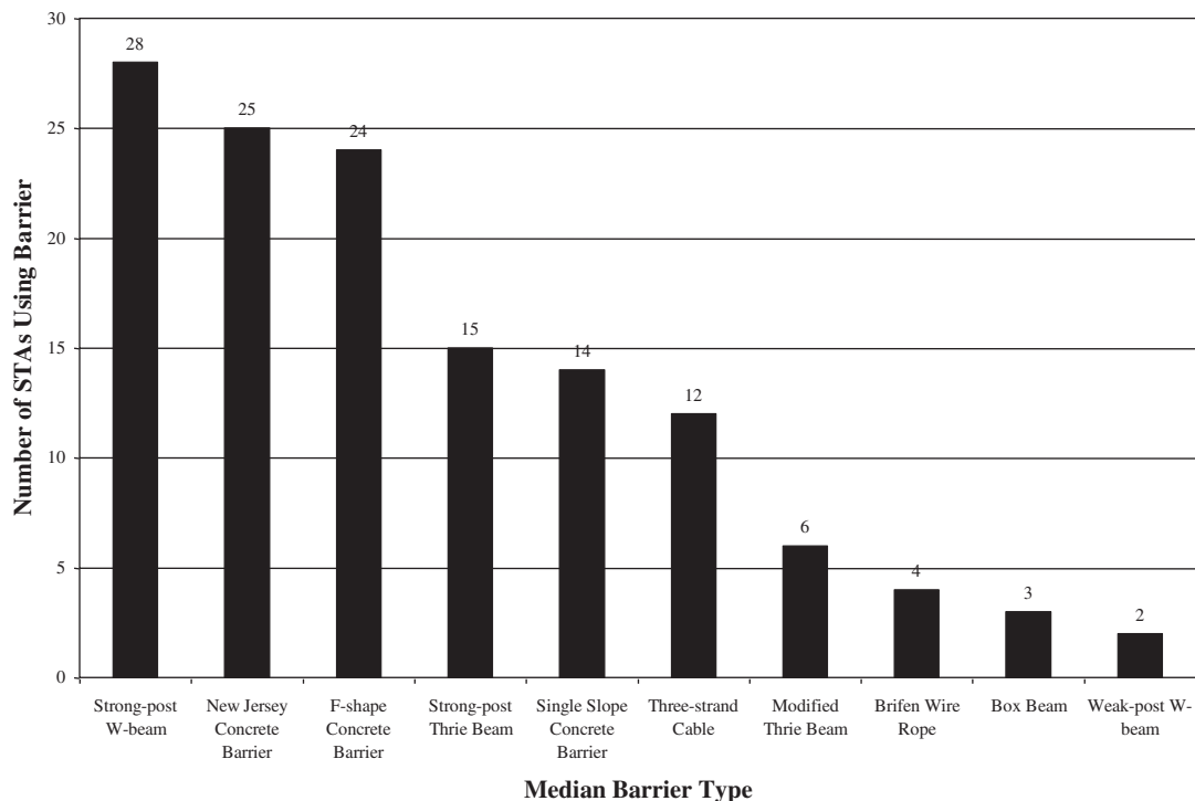
Figure 2-12. Approved median barrier use by state transportation agencies (25).
