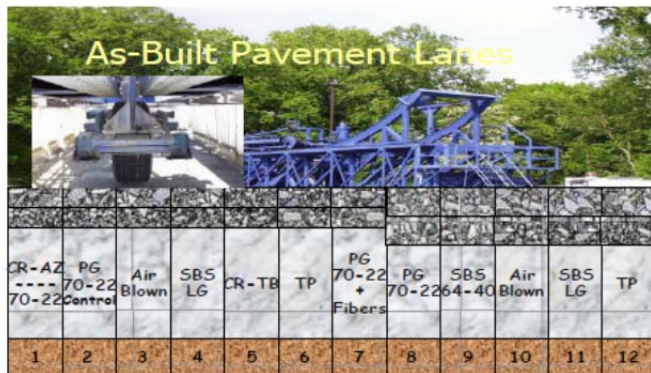
FIGURE 9 FHWA ALF test lanes and observed fatigue cracking on Lanes 2 through 6 (22).
