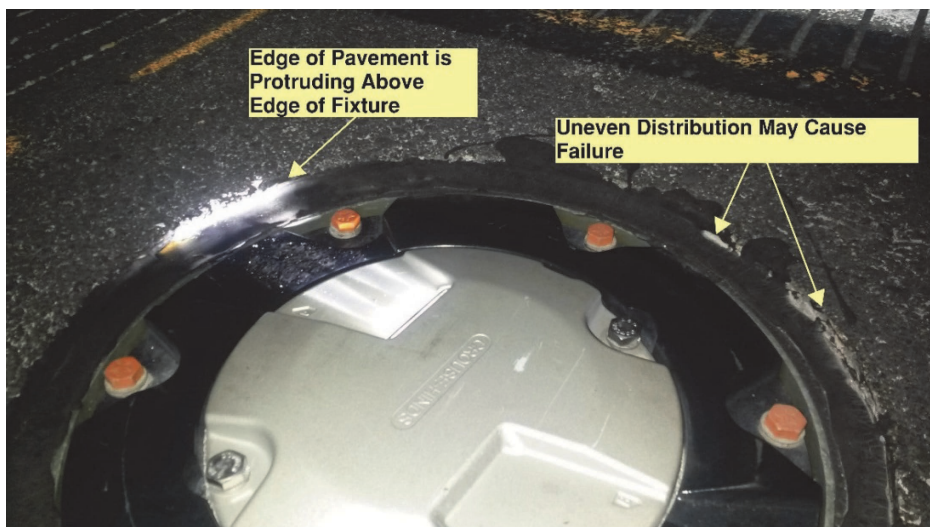
Figure 10. In-pavement fixture—visual inspection 2.
