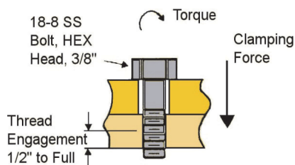
Figure 11. Mounting bolt parameters.
