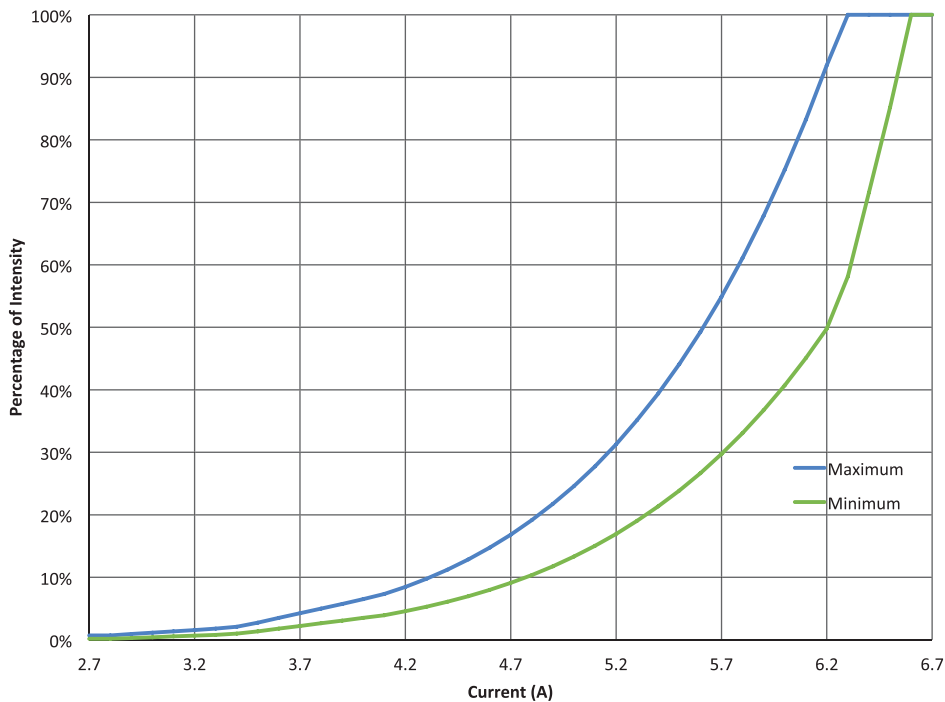
Figure 39. LED fixtures dimming curve for white LED.
