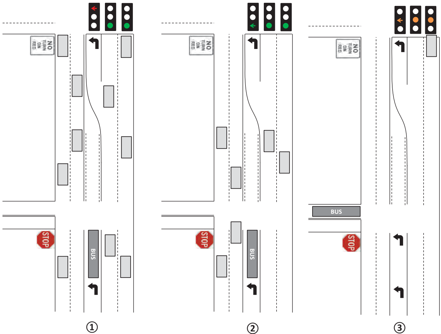
Figure 2. Example of traffic signal shadowing.
