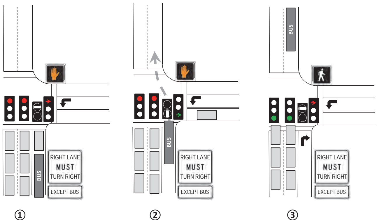
Figure 6. Illustrative example of queue jump operation from a right-turn lane with a near-side stop.
