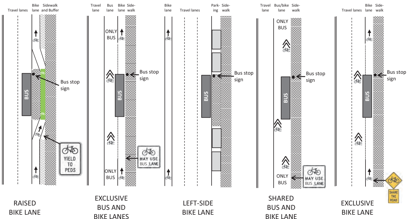
Figure C-2. Illustrative design concepts for accommodating bus and bicycle traffic.
