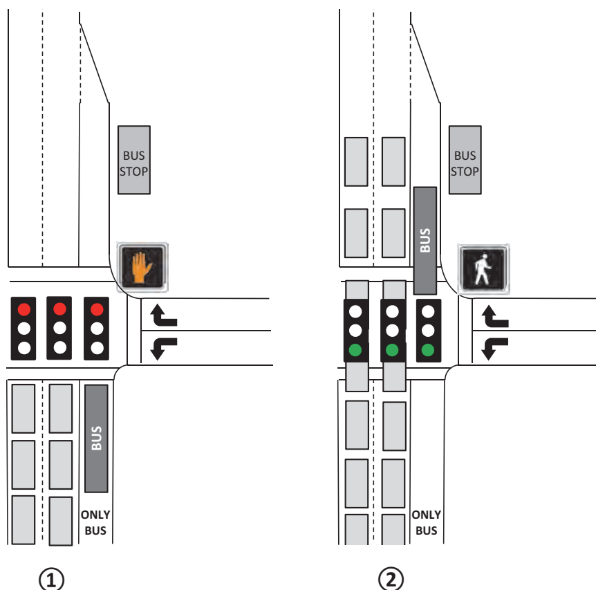
Figure 7. Illustrative queue jump operation from a short bus lane with a far-side stop.
