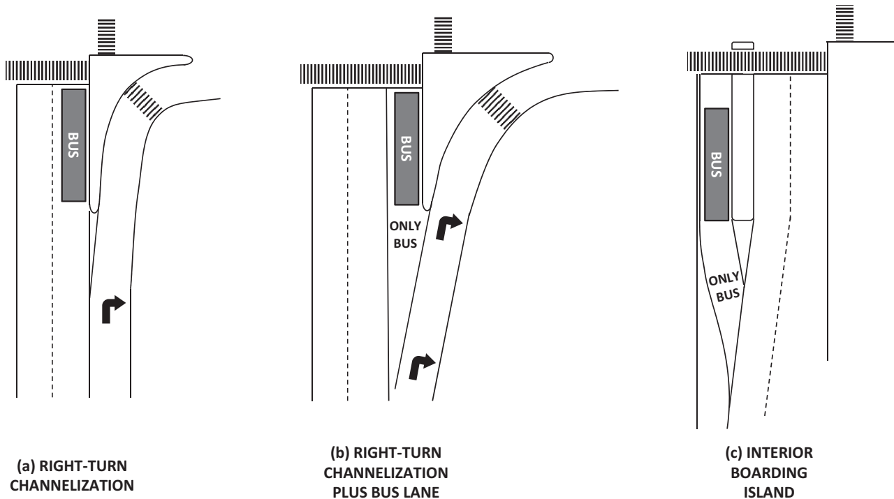
Figure 9. Illustrative boarding island configurations.
