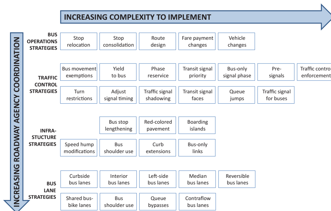
Figure S-2. Transit-supportive roadway strategies presented in this guidebook.
