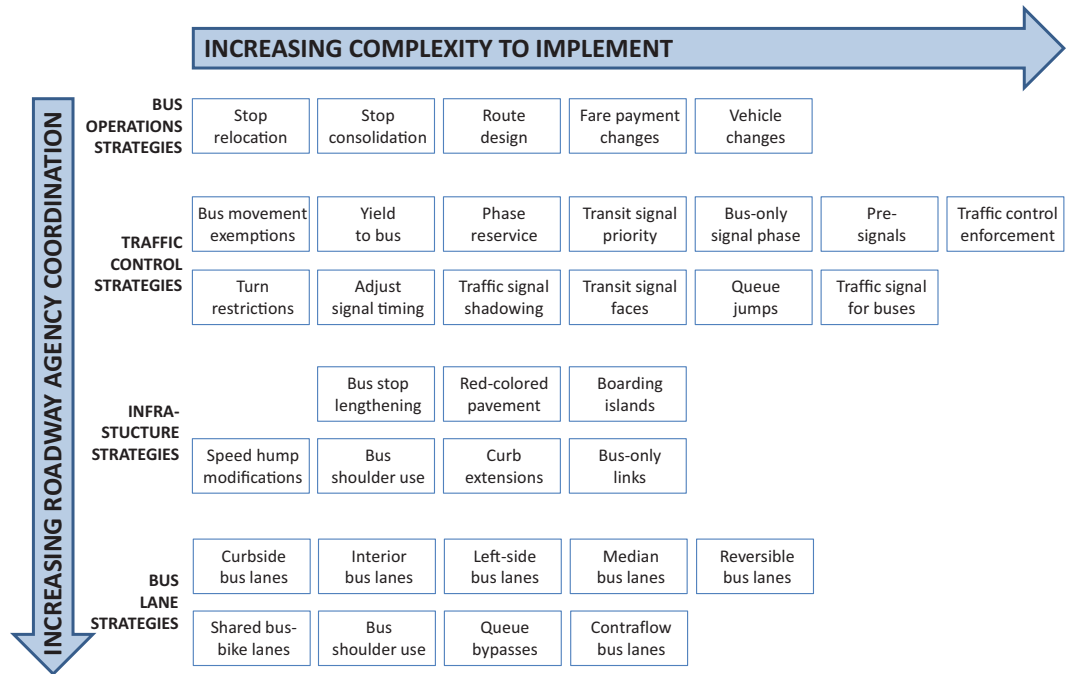
Figure 1. Transit-supportive roadway strategies categorized.
