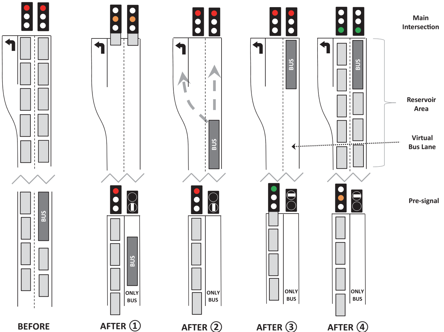
Figure 8. Examples of virtual bus lane and weave-assist applications for pre-signals.
