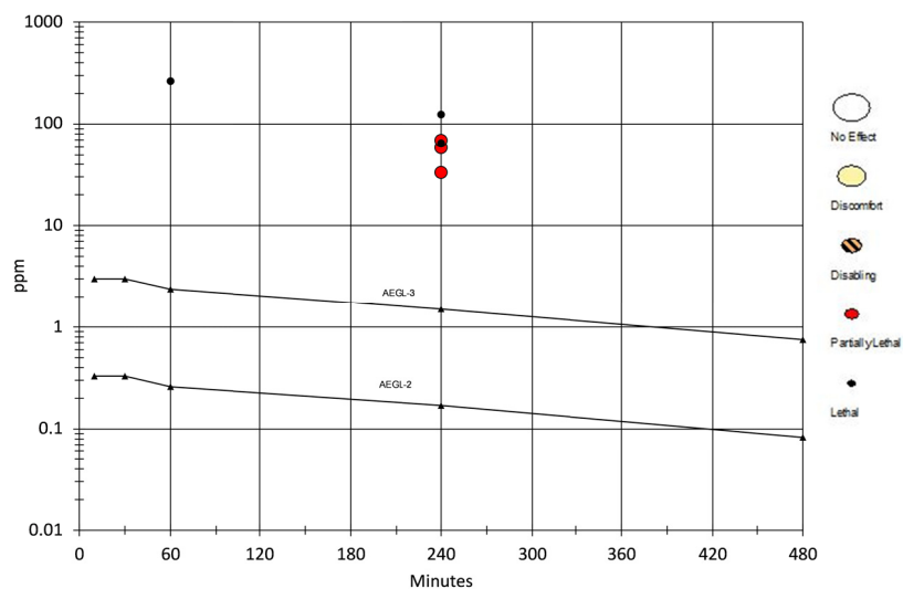
FIGURE E-10 Category plot of toxicity data and AEGL values for ethyl chloroethioformate.
