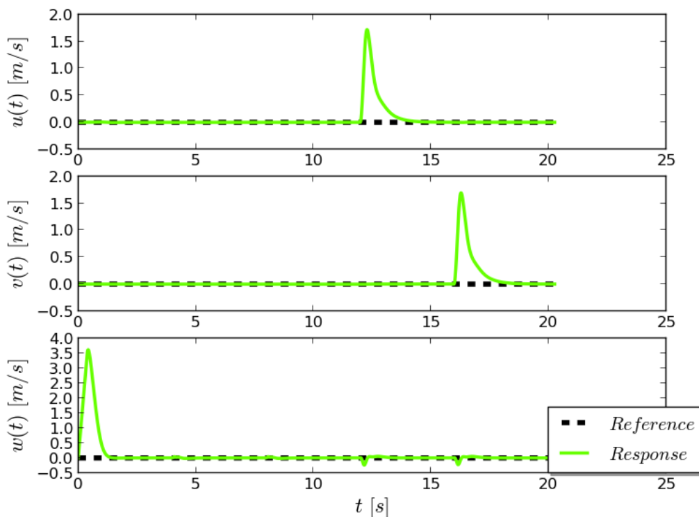
Figure 5.6: Linear velocities of the simulated platform.
