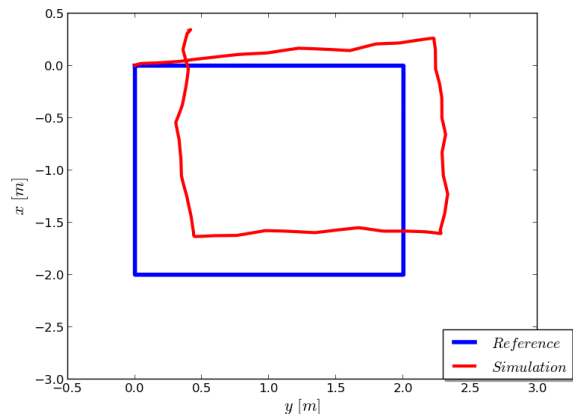
(a) Trajectory of the simulated quadrotor in the XY plane.
