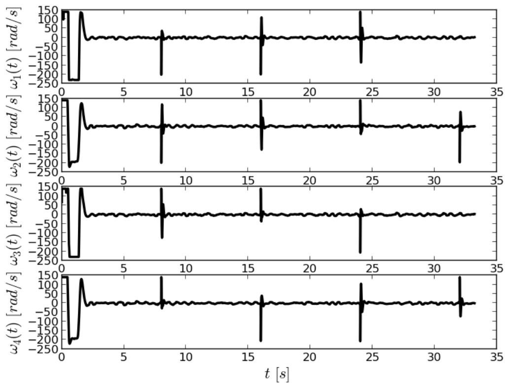
Figure 5.16: Calculated inputs from the MPC to the simulated quadrotor when using the square trajectory.
