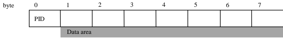
Figure 2.6 Structure for the DAQ-DTO message.
