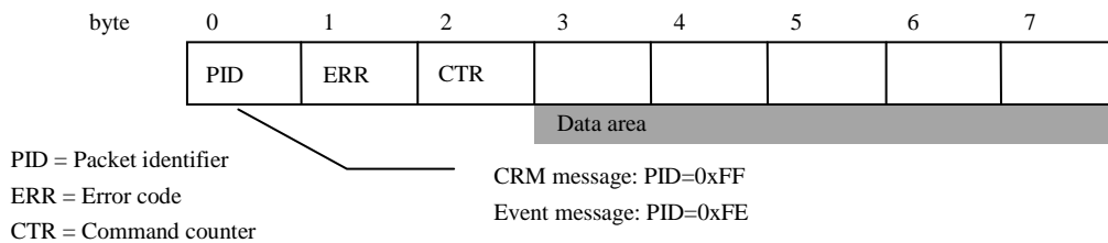
Figure 2.4 Structure for the CRM and for the event message.
