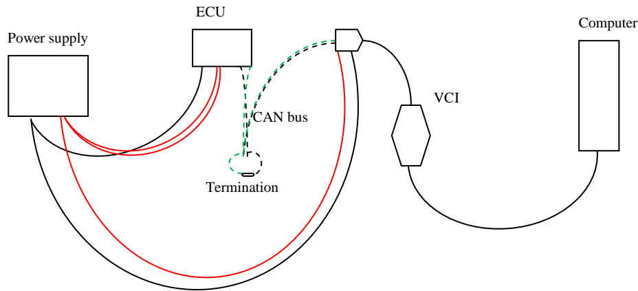
Figure 3.1 Experimental setup.
