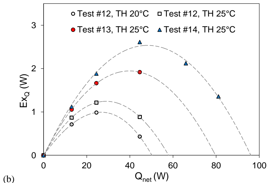
Figure 29: PMTA-1 (a) and PMTA-2 (b) results presented as exergetic cooling potential versus net cooling power.
