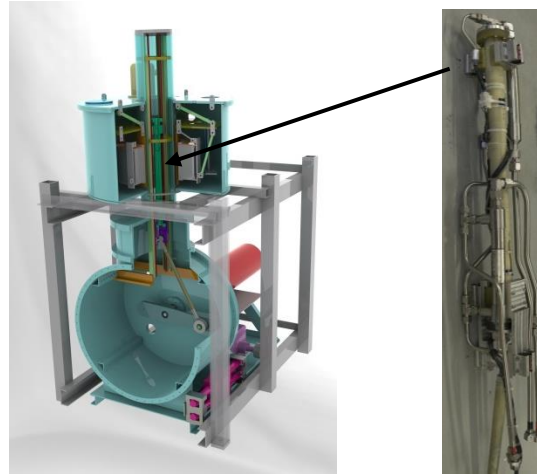
Figure 14: Rendering of SCMTA and photograph of the regenerator housing.
