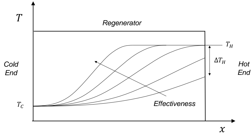
Figure 1: Example of various temperature profiles across a regenerator during a cold blow. The variability is dependent on the regenerator effectiveness which goes up according to the arrow.
