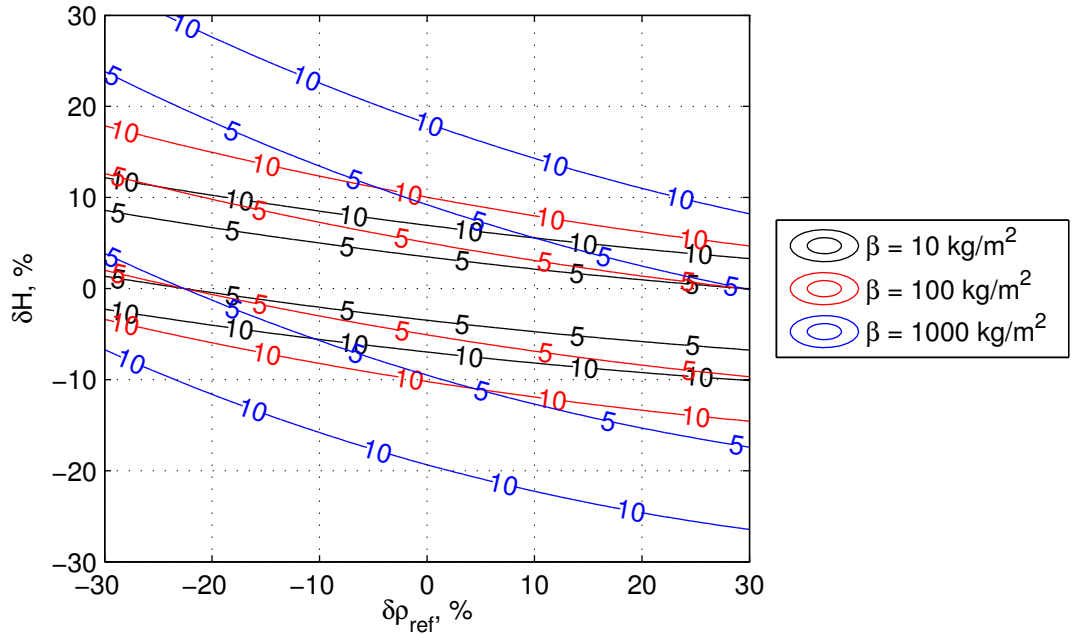
Figure 91: Combined first and second-order change in final range in km for various \beta with respect to perturbations in H and \rho_{ref} .
