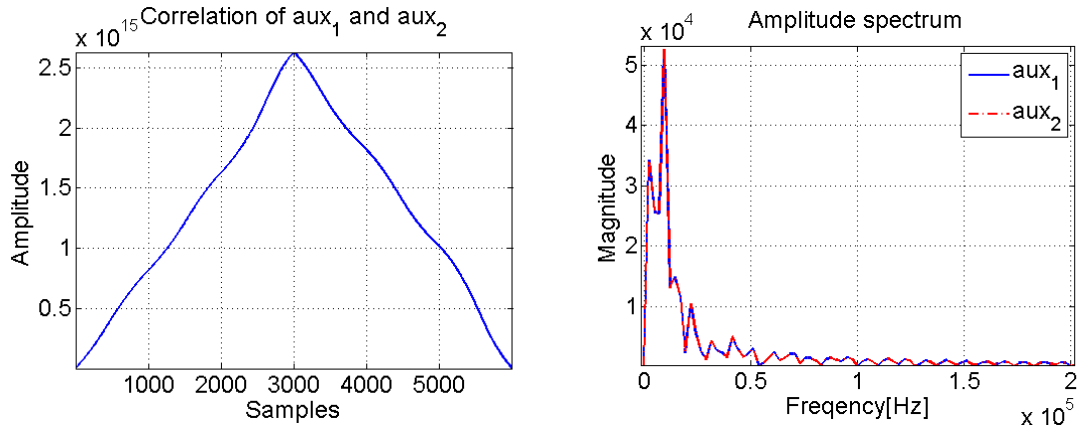
Fig. 3-17: The correlation of the auxiliary signals aux_1 and aux_2 (left) and their amplitude spectrum (right)
