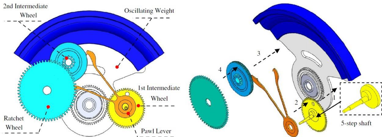
Figure 1.5 – Pawl lever mechanism [19]
