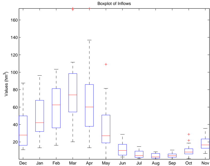
Figure 3.4: Inflows (December–November)
