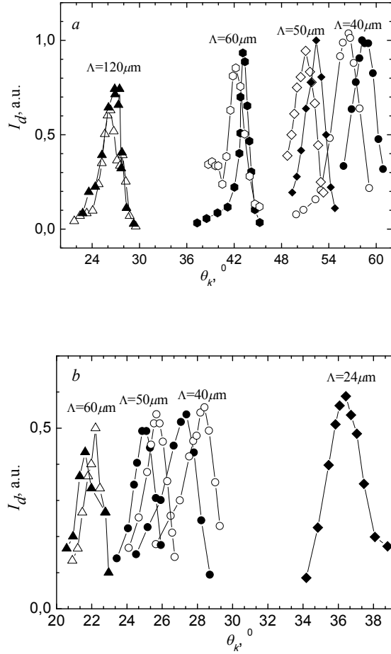
Fig. 5. The relative diffracted light intensity dependencies on polarized light incidence angle for various leaky SAW frequencies in LiNbO 3 ( a and b correspond to configuration of Fig. 1 a and b , respectively). Full dots denote ordinary incident and extraordinary diffracted, empty dots – extraordinary incident and ordinary diffracted light.
