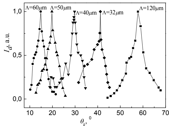
Fig. 6. The relative extraordinary diffracted light intensity dependencies on ordinary light incidence angle for various leaky SAW frequencies in LiNbO 3 (120 μm IDTs correspond to configuration of Fig. 3 a and Fig. 4 a , other IDTs – to Fig. 3 b and Fig. 4 b ).
