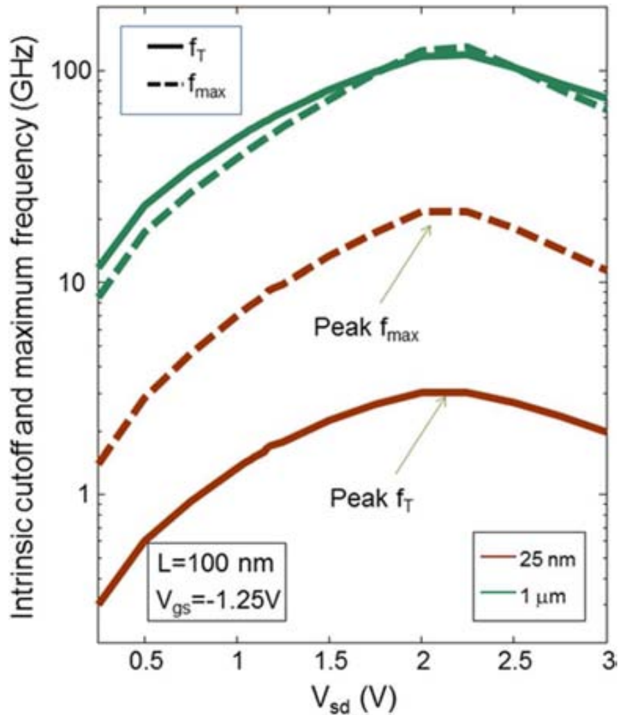
Figure 4.29: Intrinsic maximum and cutoff frequency for the simulated transistor assuming a channel length of 100\text{nm} .
