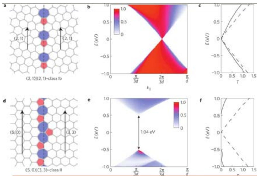
Figure 2.10: Two classes of electron transport through grain boundaries (Fig. is taken from [7])
