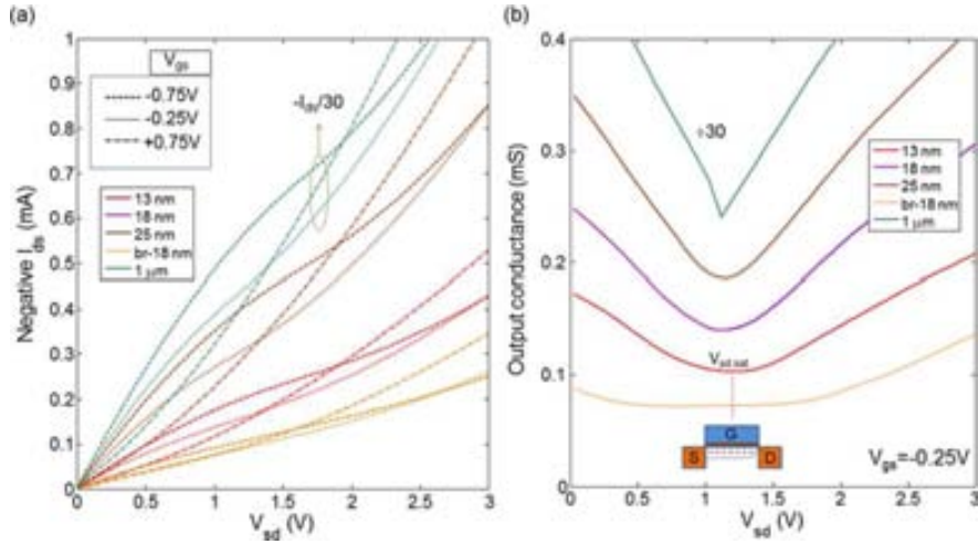
Figure 4.27: Output characteristics (a) and output conductance (b) of the graphene field-effect transistor considering different samples of polycrystalline graphene as the active channel.
