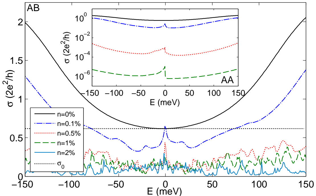
Figure 4.5: Main frame: Conductivity for strips with W = 150 nm, L = 15 nm and compensated vacancy density up to 2%. Inset: Same information for uncompensated vacancies with densities up to 1%.
