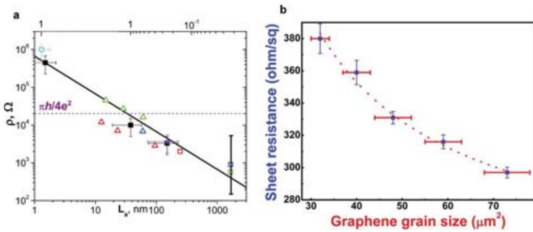
Figure 4.19: Global measurements from scaling law. a) Sheet resistance of polycrystalline graphene as a function of average grain size. Grain sizes were determined via Raman spectroscopy. Reproduced with permission. [27] Copyright 2011, IOP Publishing. b) Another example of the scaling behavior of polycrystalline graphene. The dotted line represents a fit to the scaling law described in the main text. Reproduced with permission. [18] Copyright 2012, Nature Publishing Group.
