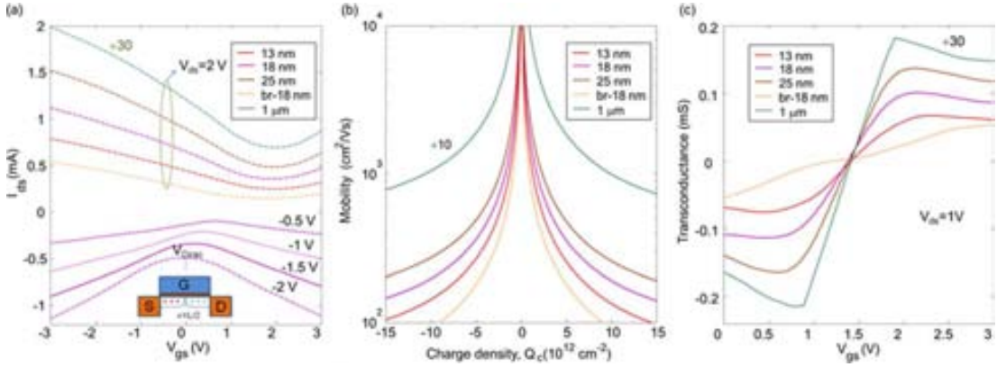
Figure 4.26: Transfer characteristics (a) and transconductance (c) of the graphene field-effect transistor considering different samples of polycrystalline graphene as the active channel. (b) Estimated low-field carrier mobility as a function of the carrier density for each of the samples.
