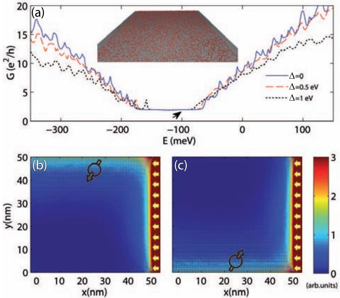
Figure 5.9: (a) Differential conductance for an armchair ribbon of width W=50 nm with a concentration n=15\% of randomly scattered thallium adatoms over a section with length L=50 nm. The potential energy on the contacts is set to V=-2.5 eV. The presence of long-range disorder with \Delta up to 1 eV is taken into account. (b) Local density-of-occupied-states for spin down electrons injected from the right contact for \Delta = 0 at energy E=-100 meV, see the arrow in (a). (c) Same as (b) but for spin up electrons.
