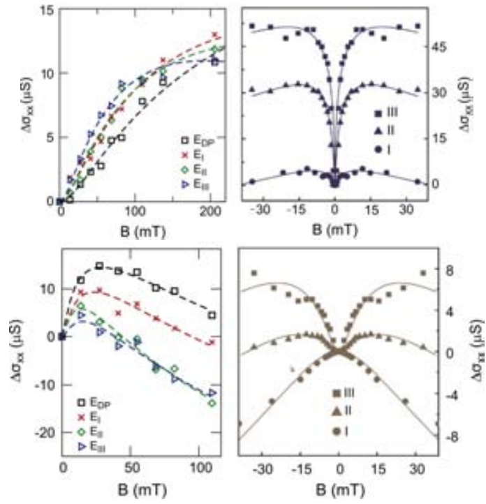
Figure 2.6: Magnetoconductance for W = 2\gamma_0 (top panels) and W = 1.5\gamma_0 (bottom panels), the data is extracted from theoretical (left panels) and experimental (right panels) study (Fig. is taken from [4])
