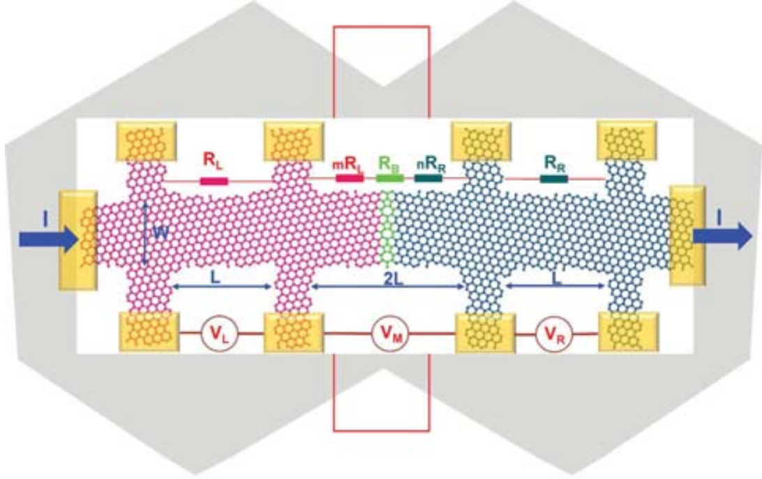
Figure 4.16: Principle of four-probe measurement applied to GGBs. A series of Hall bars is fabricated across the GGB region. The resistivity of the GGBs can be extracted from this measurement set-up. Intra-grain resistances R_L and R_R are subtracted from the inter-grain resistance to obtain R_B , the resistance of the GGB.
