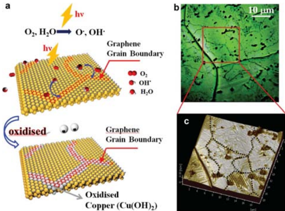
Figure 4.11: UV treatment approach to identifying graphene grain orientations. a) Principle of GGB visualization by UV treatment. b-c) Selective oxidation of an underlying the copper substrate for direct optical identification (b) of the GGBs, confirmed by AFM (c). Reproduced with permission. [18] Copyright 2012, Nature Publishing Group.
