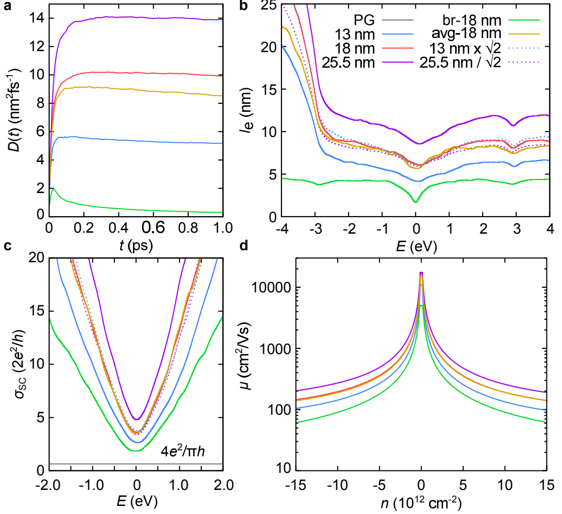
Figure 4.14: (a) Diffusion coefficient ( D(t) ) for the samples presented in Fig. 4.12. (b) Mean free path \ell_e(E) for equivalent structures with scaled \ell_e(E) for samples with \langle d \rangle \approx 13 nm and \langle d \rangle \approx 25.5 nm, showing the scaling law. (c) Semi-classical conductivity ( \sigma_{\text{sc}}(E) ) for all samples and as scaled for the same cases as above. (d) Charge mobility ( \mu(E) = \sigma_{\text{sc}}(E)/en(E) ) as a function of the carrier density n(E) in each of the samples ( n(E) = 1/S \int_0^E \rho(E)dE , S being a normalization factor).
