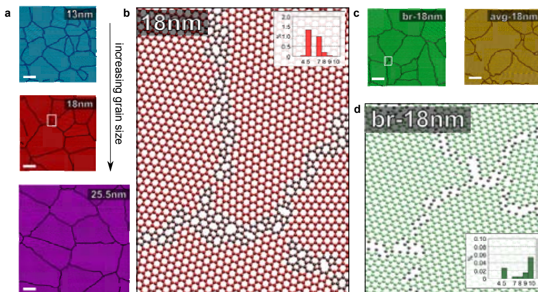
Figure 4.12: (a) Three structures with uniform grain size distribution and increasing average grain sizes (13.0, 18.0 and 25.5 nm). GBs are marked with dark lines. (b) Larger magnification of the area marked with a white rectangle in panel (a), showing a typical example of the grain boundaries. Carbon ring-size statistics for the same sample (showing the ratio of non-hexagonal rings) are presented in the upper right corner. (c) Two additional samples with average grain size of 18 nm: one sample with broken boundaries (“br-18 nm”) and another one with random grain size distribution (“avg-18 nm”). (d) Higher magnification of the area marked with a white rectangle in panel (c), showing the structure of “broken” boundaries in sample “br-18 nm”. The statistics of non-hexagonal rings are shown in the lower right corner. All scale bars are 10 nm.
