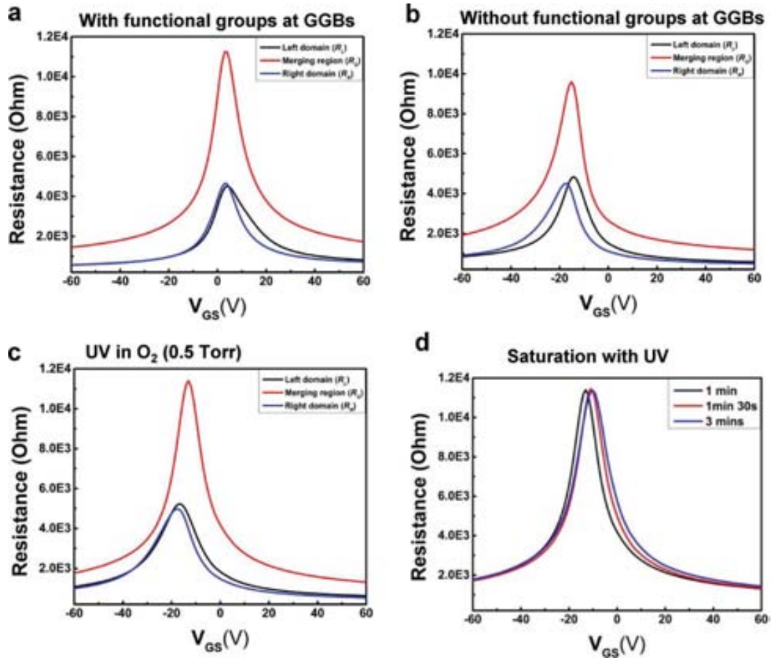
Figure 4.22: O_2 Selective functionalization of GGBs by UV treatment under environment. a)-b) Effect of annealing at 250^\circ C in 3h. Functional groups are removed from a GGB. c)-d) Effect of UV treatment under O_2 environment. The exclusive change of the inter-grain resistance indicates selective functionalization at the GGB. The UV treatment is saturated after 1 minute of UV treatment.
