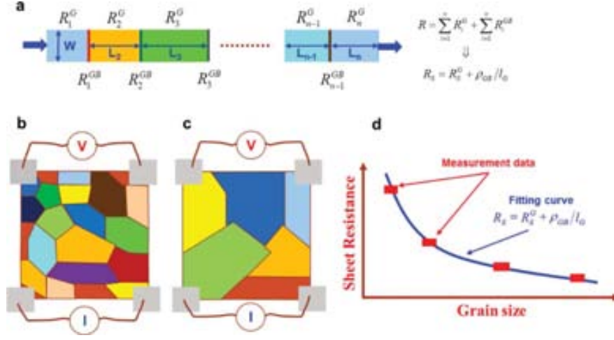
Figure 4.18: Principle of the scaling law to extract the GGB resistivity. a) Derivation of the ohmic scaling law. b)-c) Sheet resistance measurements of graphene with small and large grain sizes. d) Extraction of GGB resistivity by fitting the scaling law to sheet resistance measurements.
