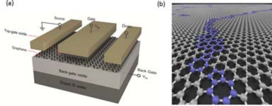
Figure 4.24: (a) Schematic of the dual-gate GFET, consisting of a poly-G channel on top of an insulator layer, which is grown on a heavily-doped Si wafer acting as the back gate. An artistic view of the patchwork of coalescing graphene grains of varying lattice orientations and size is shown in (b). The source and drain electrodes contact the poly-G channel from the top and are assumed to be ohmic. The source is grounded and considered the reference potential in the device. The electrostatic modulation of the carrier concentration in graphene is achieved via a top-gate stack consisting of the gate dielectric and the gate metal.
