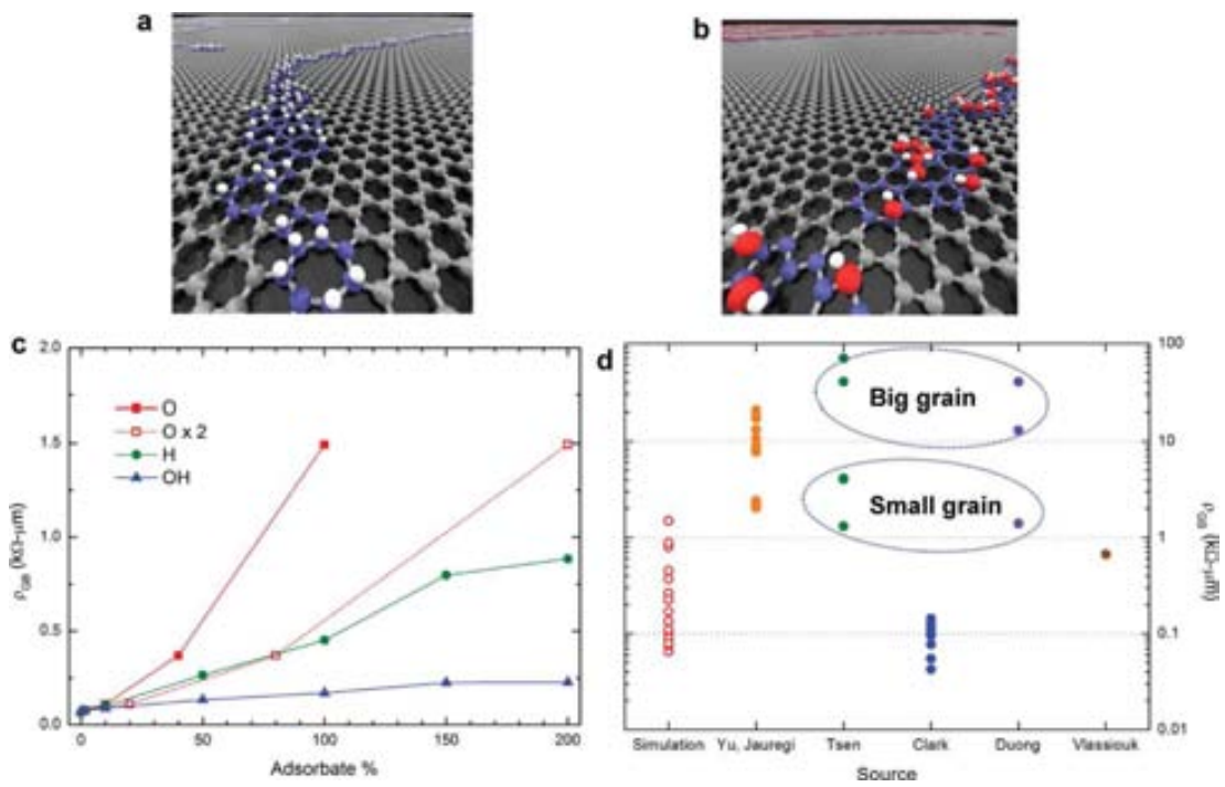
Figure 4.23: Simulation of the effect of functional groups at GGBs. a)-b) Schematic of GGBs functionalized by H and OH groups, respectively. c) Dependence of the resistivity of GGBs on functional groups with various concentrations. d) Summary of experimental and simulated results for the resistivity of GGBs.
