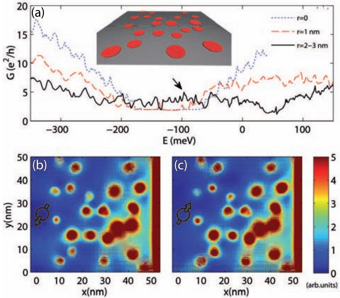
Figure 5.10: (a) Differential conductance for an armchair ribbon of width W=50 nm with a concentration n=15\% of clustered thallium adatoms (in islands with radius r up to 2-3 nm) over a section with length L=50 nm. The potential energy on the contacts is set to V=-2.5 eV. (b) Local density-of-occupied-states in the case r \in [2, 3] nm, for spin down electrons injected from the right contact at energy E=-100 meV, see the arrow in (a). (c) Same as (b) but for spin up electrons.
