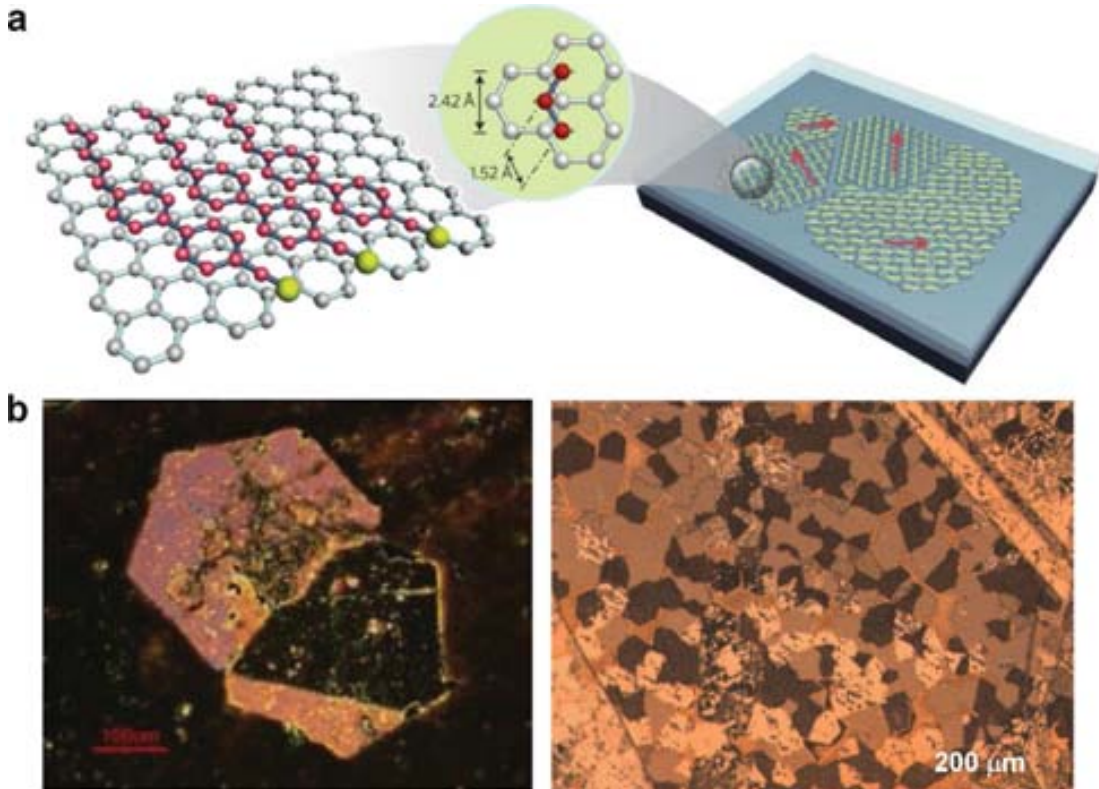
Figure 4.10: Liquid crystal coating approach to identifying graphene grain orientations. a) The hexagonal rings of LC molecules align coherently with hexagonal rings in graphene. Reproduced with permission. [22] Copyright 2012, Nature Publishing Group. b) POM images of LC molecules aligned on each graphene grain, revealing a strong optical contrast between misoriented grains.
