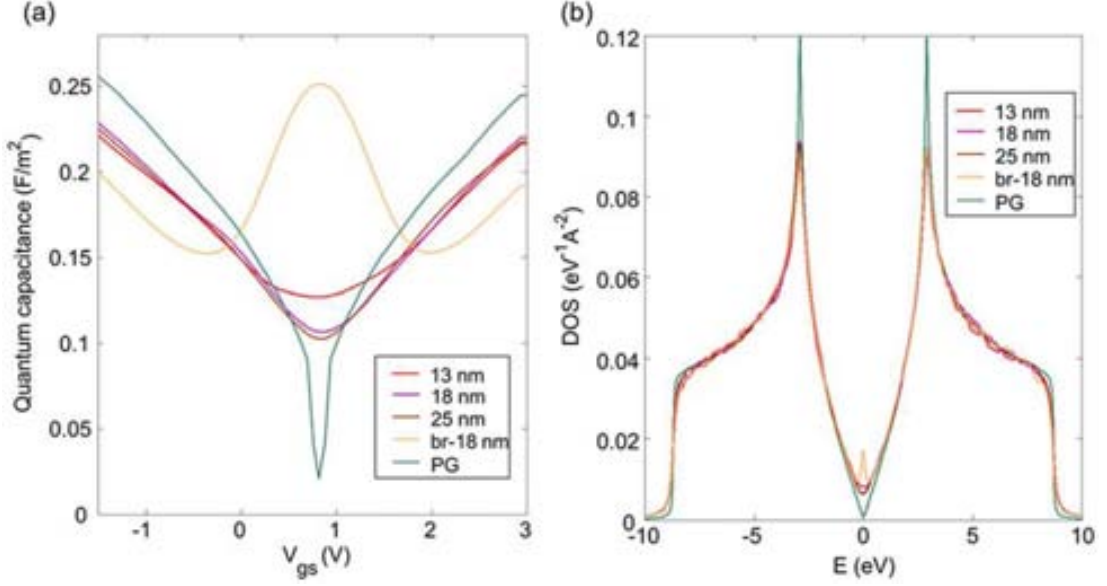
Figure 4.25: Quantum capacitance (a) and density of states (b) of polycrystalline graphene considering different average grain sizes. The PG case has also been plotted for the sake of comparison.
