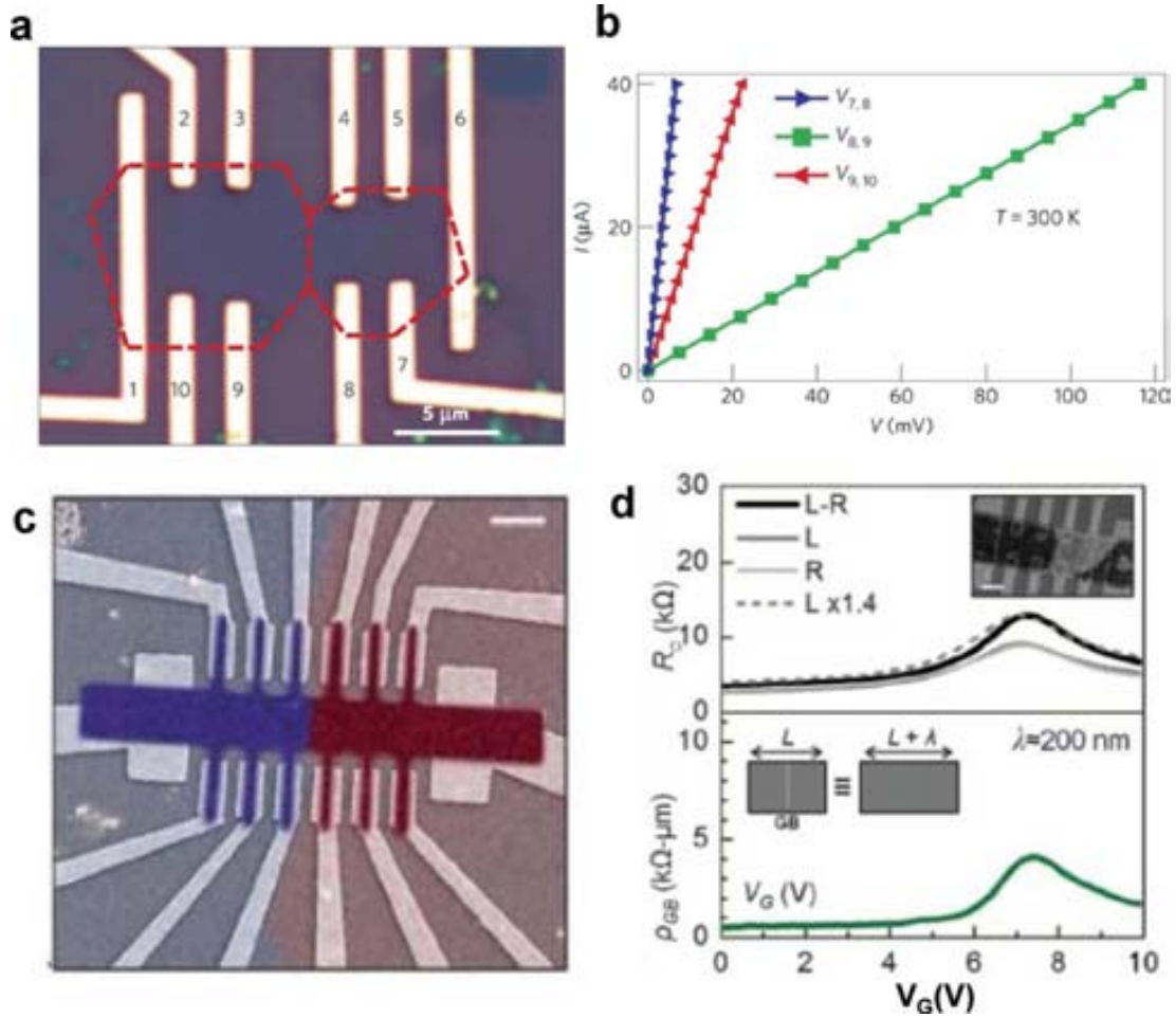
Figure 4.17: Four-probe measurement of GGBs. a) Example of a four-probe setup for measuring the resistivity of a GGB. b) I-V curves measured within individual grains (red and blue curves) and across the GGB (green curve). The reduced slope for the inter-grain measurement indicates extra resistance contributed by the GGB. Reproduced with permission. [25] Copyright 2011, Nature Publishing Group. c) Four-probe measurement setup mounted on a TEM holder, where individual graphene grains are identified in the red and blue regions. d) Top plot; four-probe measurements of the inter- and intra-grain resistance as a function of gate voltage (black and gray curves, respectively). Bottom plot; the extracted GB resistivity as a function of gate voltage in volt. Reproduced with permission. [26] Copyright 2013, AAAS.
