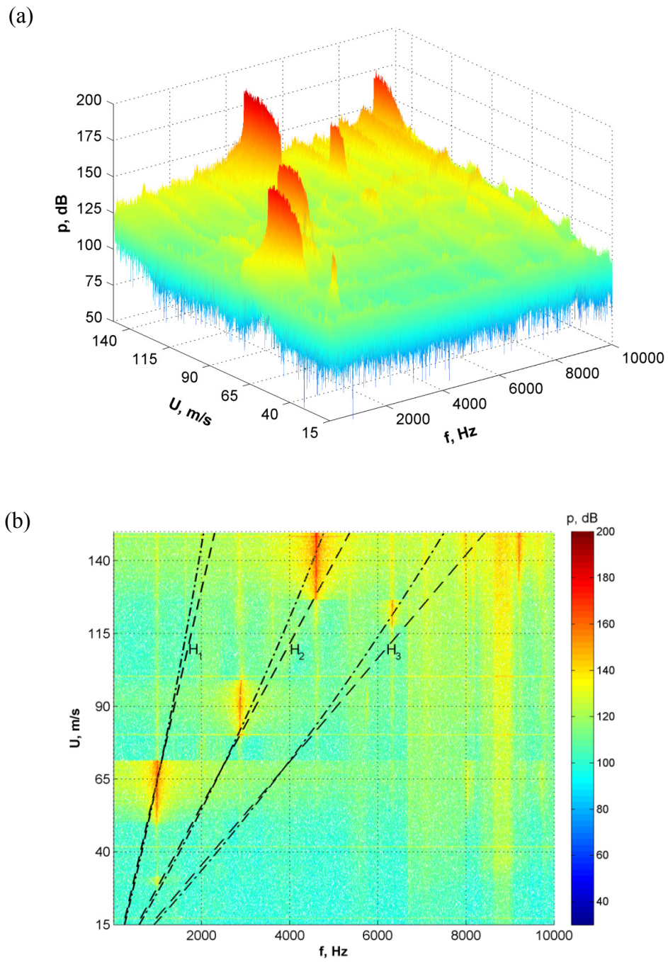
Figure 4.9: Pressure amplitude as a function of the frequency f and the inflow velocity U for the case of the downstream chamfer length L_C = 3.81 mm: (a) waterfall plot, (b) contour plot. Shear layer oscillation modes:
