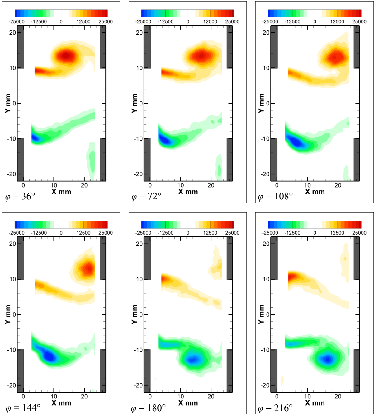
Figure B.3: Patterns of phase-averaged out-of-plane vorticity (s -1 ) corresponding to the symmetric case L_C = 1.27 mm, \varphi = 36^\circ through 216^\circ .
