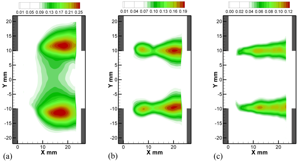
Figure 6.5: Patterns of time-averaged v_{rms}/U corresponding to the (a) first ( St = 0.37 , U = 67\text{m/s} ), (b) second ( St = 0.8 , U = 91.5\text{ m/s} ), and (c) third ( St = 1.32 , U = 121\text{ m/s} ) hydrodynamic mode for the case L_C = 0\text{ mm} .
