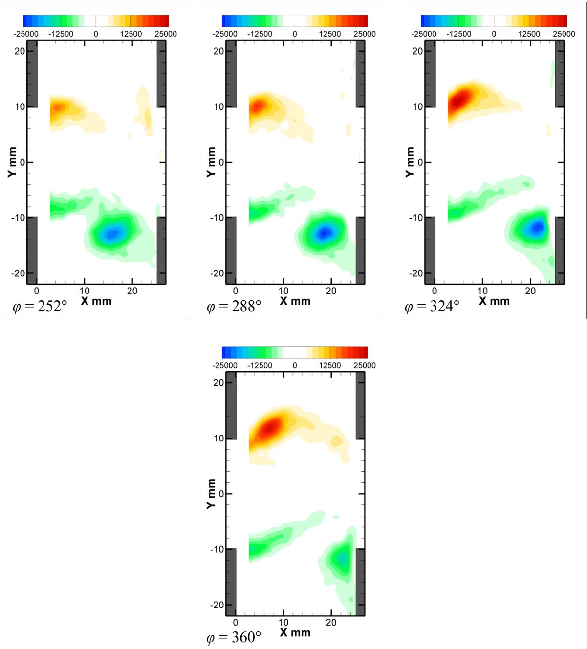
Figure B.10: Patterns of phase-averaged out-of-plane vorticity ( \text{s}^{-1} ) corresponding to the upstream case L_C = 3.81 mm, \varphi = 252^\circ through 360^\circ .
