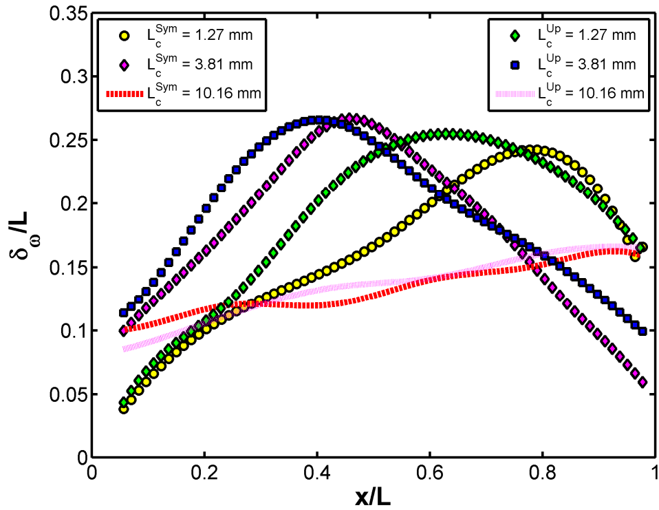
Figure 6.8: Growth of the vorticity thickness across the cavity corresponding to the case of the symmetric and upstream chamfer with chamfer length: L_c = 1.27 mm, L_c = 3.81 mm, L_c = 10.16 mm.
