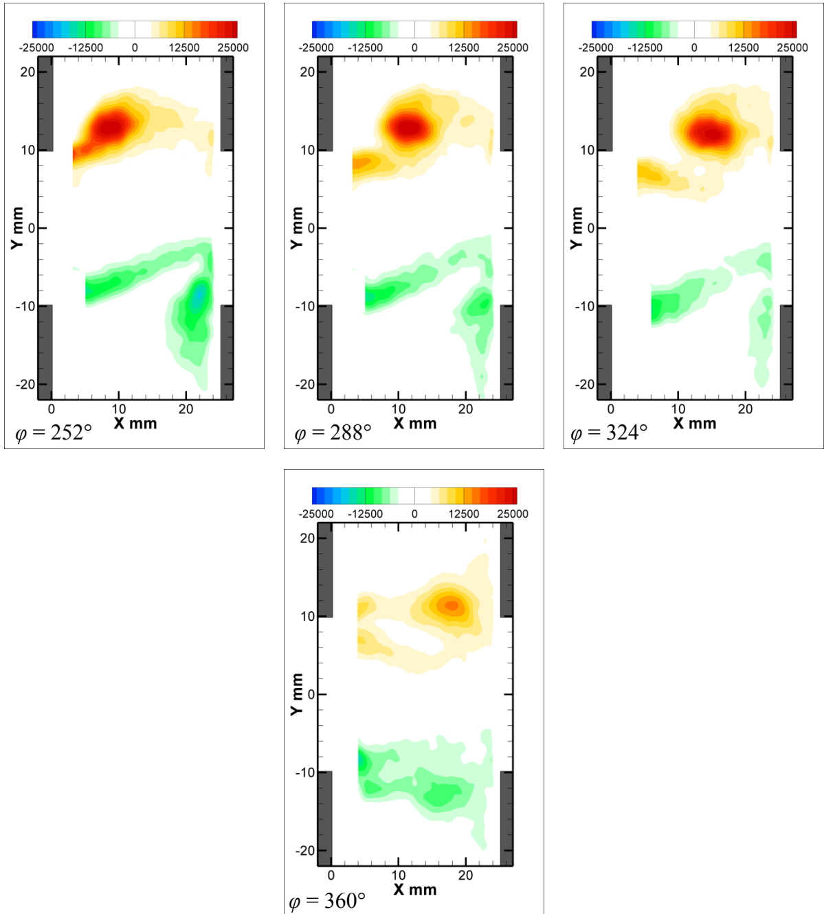
Figure B.6: Patterns of phase-averaged out-of-plane vorticity ( s^{-1} ) corresponding to the symmetric case L_C = 1.27 mm, \varphi = 252^\circ through 360^\circ .
