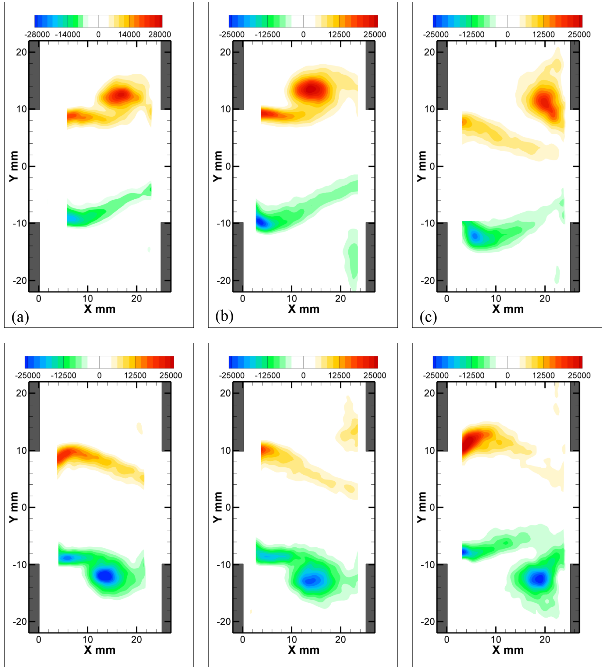
Figure 6.12: Patterns of phase-averaged out-of-plane vorticity ( s^{-1} ) corresponding to the (a) L_C = 0 ( St = 0.37 , U = 67\text{m/s} ), (b) L_C = 1.27\text{ mm} ( St = 0.36 , U = 70\text{ m/s} ), and (c) L_C = 3.81\text{ mm} ( St = 0.29 , U = 87\text{ m/s} ) at \varphi = 36^\circ and 180^\circ .
