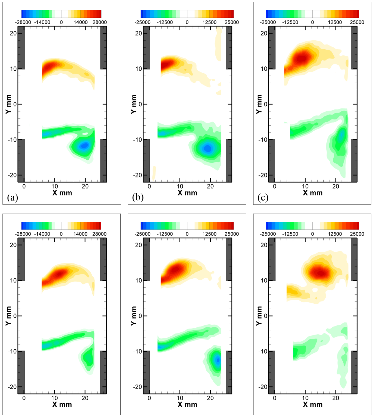
Figure 6.13: Patterns of phase-averaged out-of-plane vorticity ( \text{s}^{-1} ) corresponding to the symmetric cases (a) L_C = 0 ( \text{St} = 0.37 , U = 67\text{m/s} ), (b) L_C = 1.27\text{ mm} ( \text{St} = 0.36 , U = 70\text{ m/s} ), and (c) L_C = 3.81\text{ mm} ( \text{St} = 0.29 , U = 87\text{ m/s} ) at \varphi = 252^\circ and 324^\circ .
