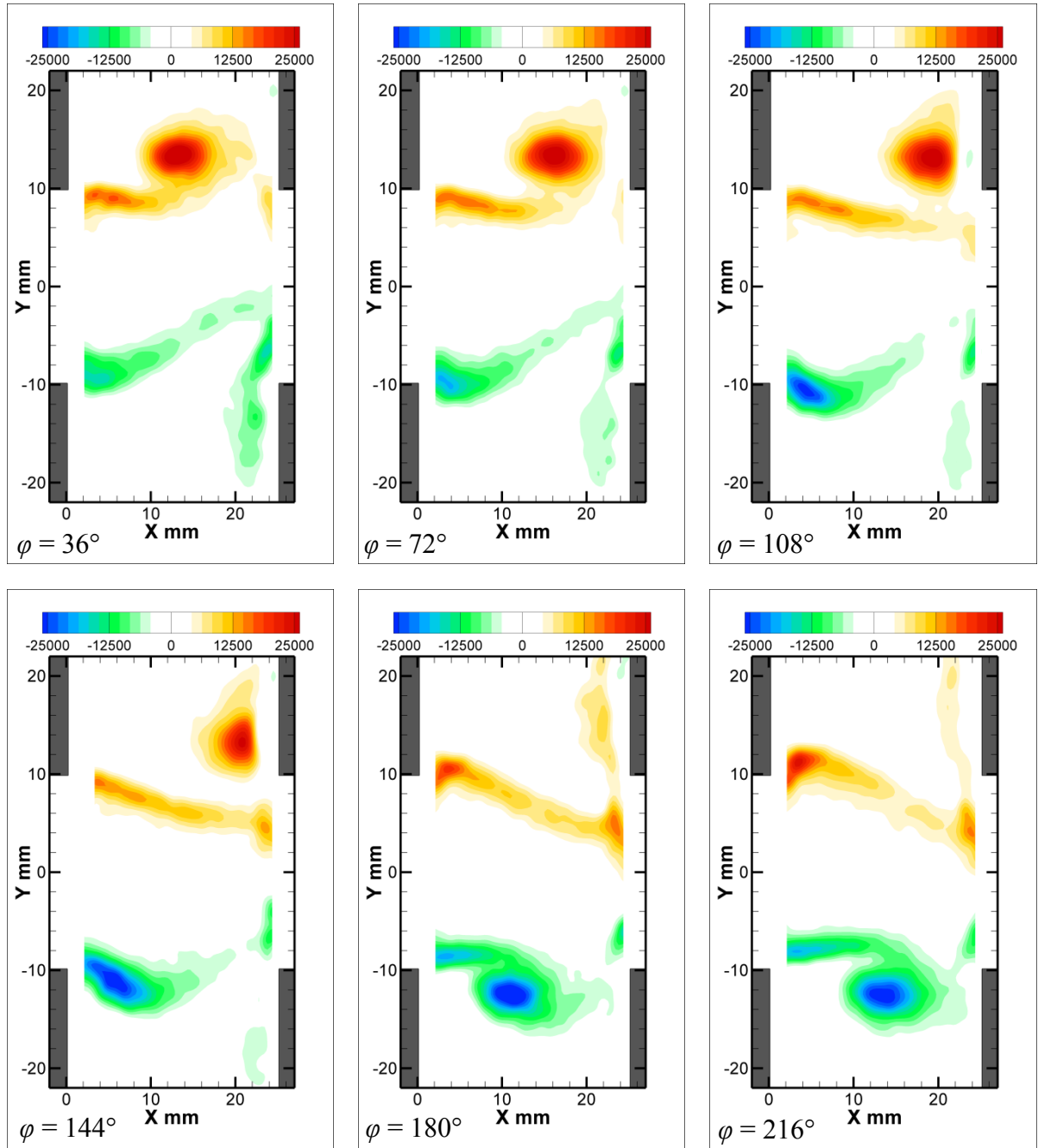
Figure B.7: Patterns of phase-averaged out-of-plane vorticity ( s^{-1} ) corresponding to the upstream case L_C = 1.27 mm, \varphi = 36^\circ through 216^\circ .
