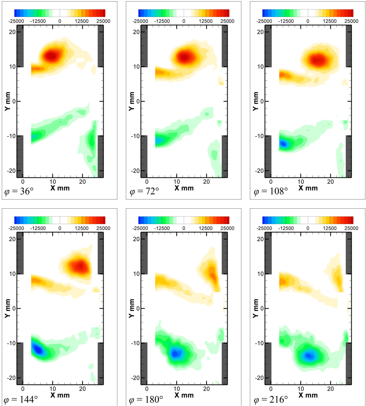
Figure B.9: Patterns of phase-averaged out-of-plane vorticity (s -1 ) corresponding to the upstream case L_C = 3.81 mm, \varphi = 36^\circ through 216^\circ .
