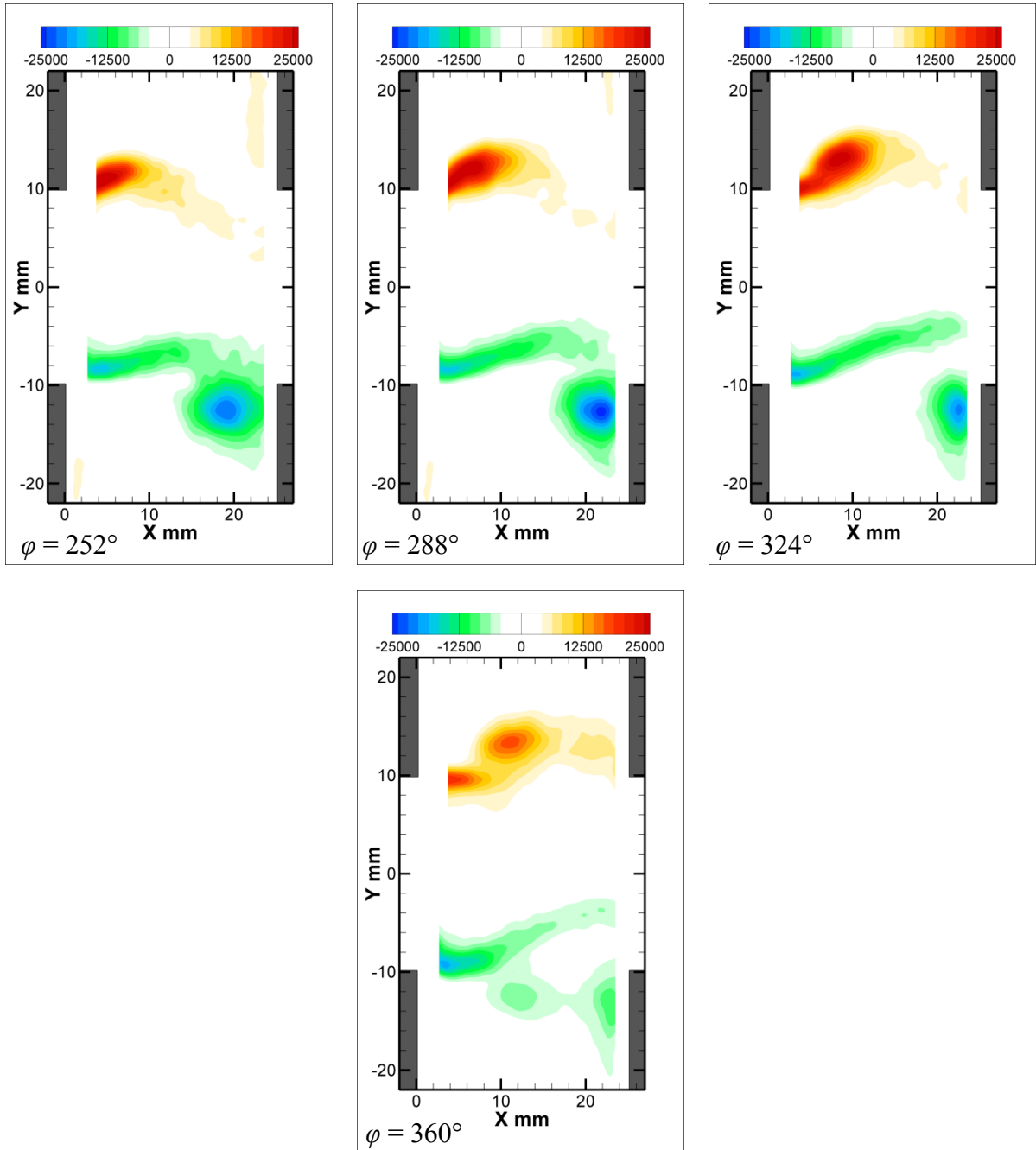
Figure B.4: Patterns of phase-averaged out-of-plane vorticity ( s^{-1} ) corresponding to the symmetric case L_C = 1.27 mm, \varphi = 252^\circ through 360^\circ .
