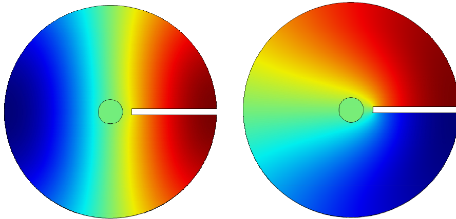
Figure 5.10: The mode shapes of the first acoustic diametral mode in the presence of the long splitter plate ( L_S = 81.4 mm): (a) f_A^1 = 998 Hz, (b) f_B^1 = 713 Hz.
