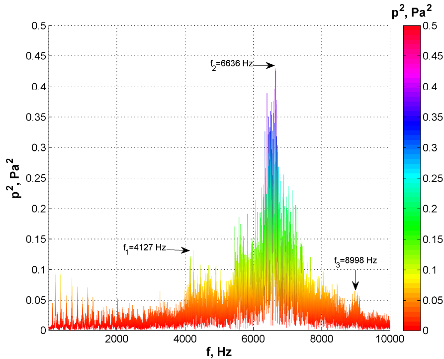
Figure 3.4: Pressure spectrum corresponding to the inflow velocity U = 21.5 m/s, for the case of \alpha = 5^\circ .
