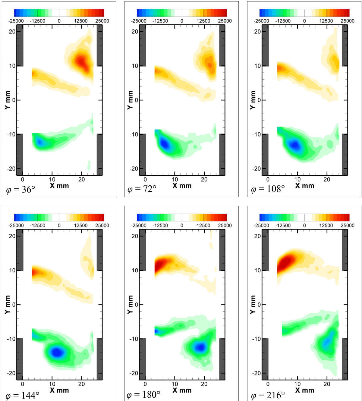
Figure B.5: Patterns of phase-averaged out-of-plane vorticity ( s^{-1} ) corresponding to the symmetric case L_C = 3.81 mm, \varphi = 36^\circ through 216^\circ .
