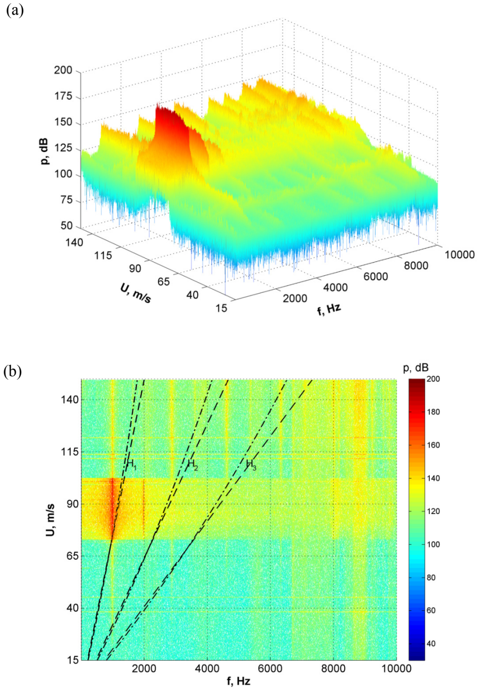
Figure 4.12: Pressure amplitude as a function of the frequency f and the inflow velocity U for the case of the upstream chamfer length L_C = 3.81 mm: (a) waterfall plot, (b) contour plot. Shear layer oscillation modes:
