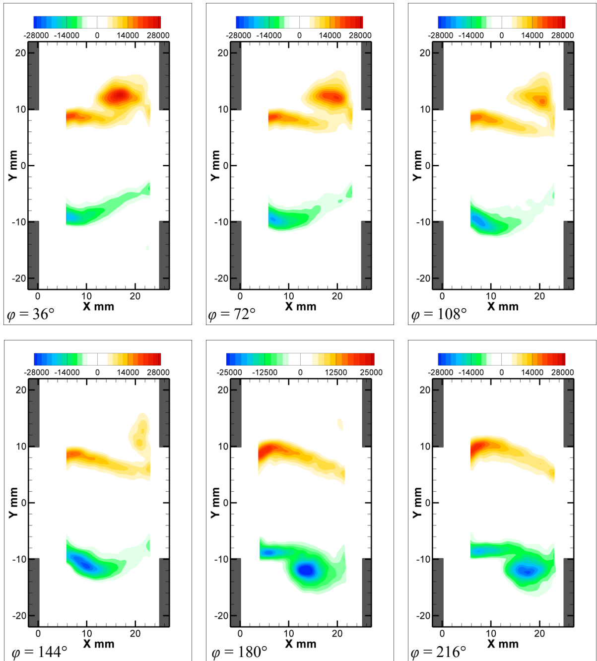
Figure B.1: Patterns of phase-averaged out-of-plane vorticity ( s^{-1} ) corresponding to the symmetric case L_C = 0 , \varphi = 36^\circ through 216^\circ .
