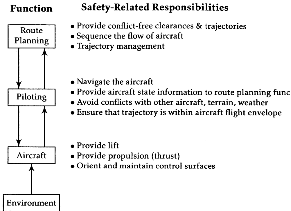
Figure 16: High Level Control Structure & Responsibilities
