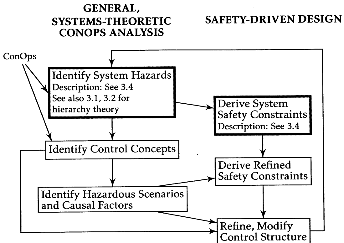
Figure 15: Methodology—Top-Level Systems Engineering
