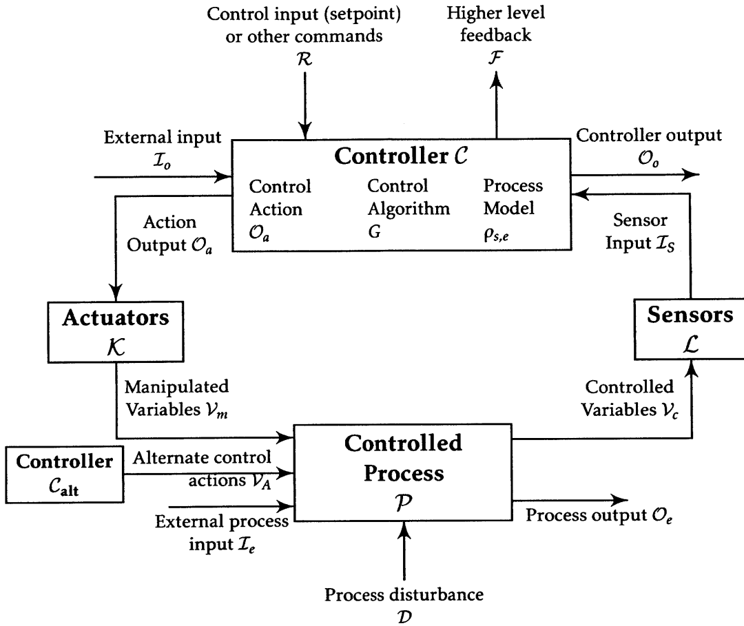
Figure 13: Generic Process Control Loop
