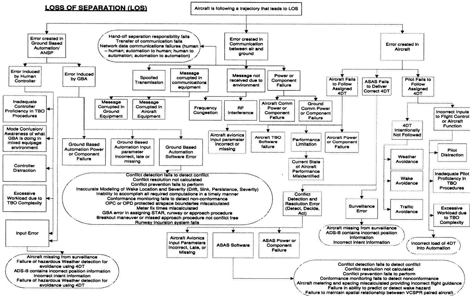
Figure 33: Loss of Separation Fault Tree Analysis [JPDO, 2012]
