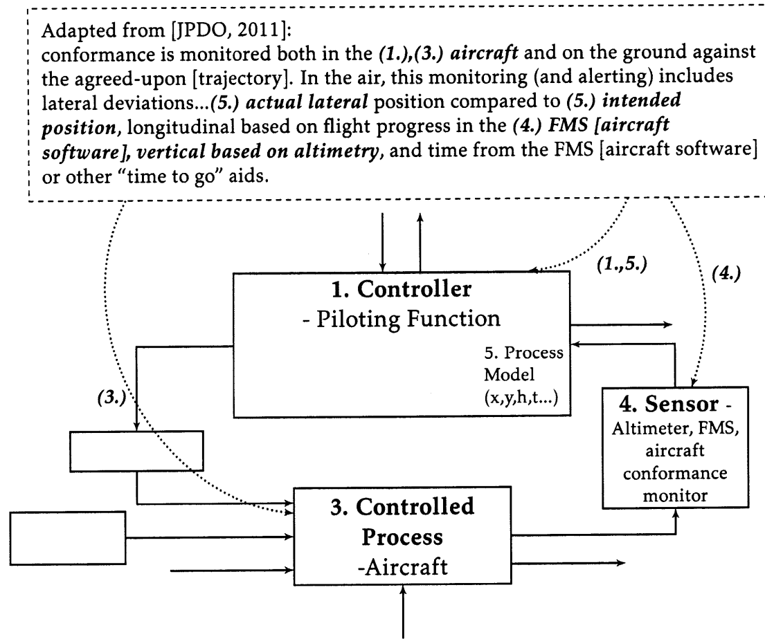
Figure 18: Graphical Control Model of Airborne Conformance Monitor
