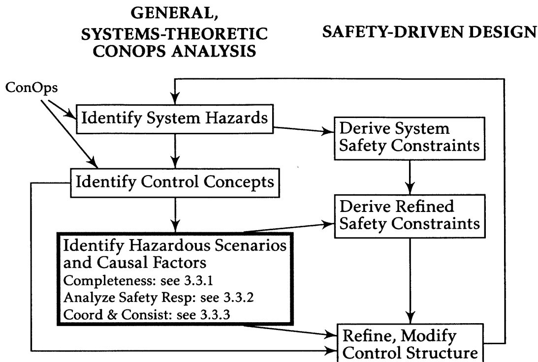
Figure 22: Methodology—Identifying Hazardous Scenarios
