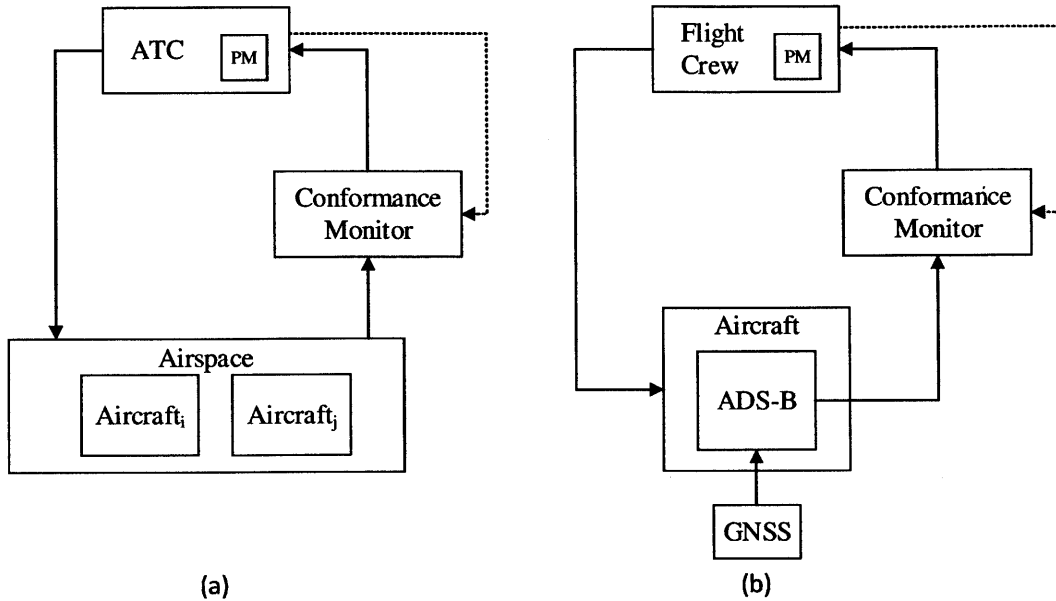
Figure 20: Individual Control Loops derived via Analysis
