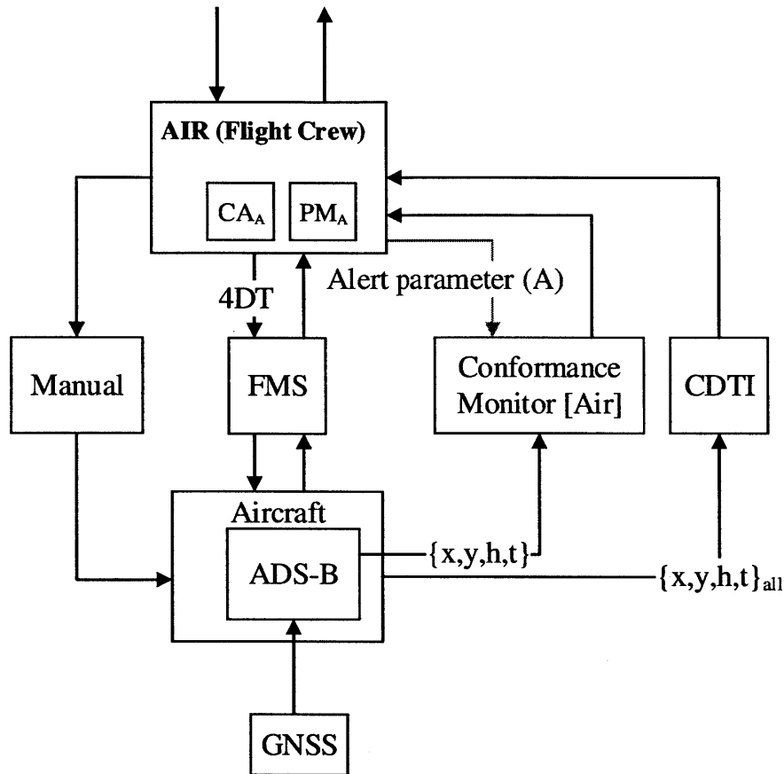
Figure 36: Flight Deck (Airborne) Control Loops
