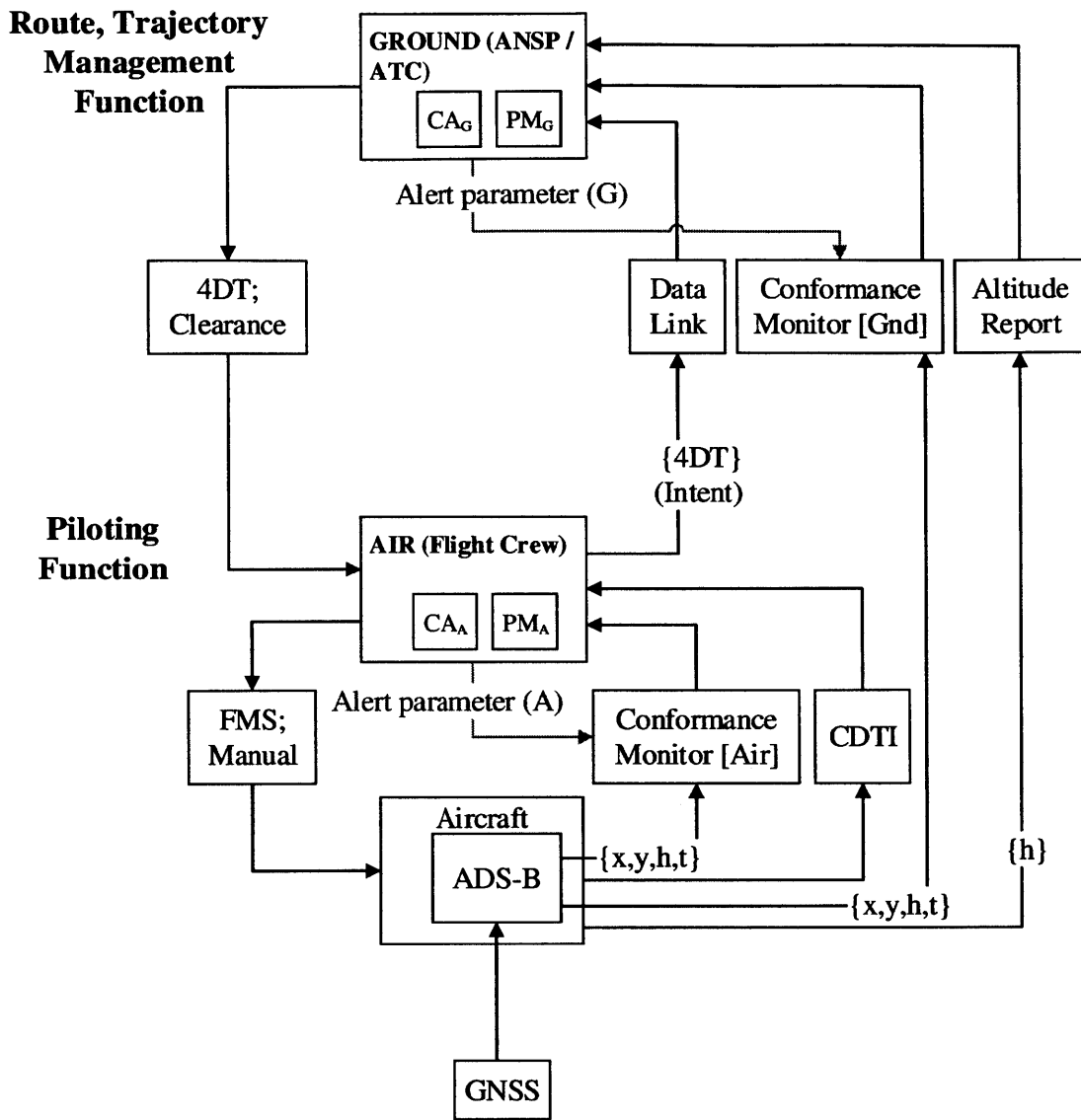
Figure 35: General Conformance Monitoring System Model
