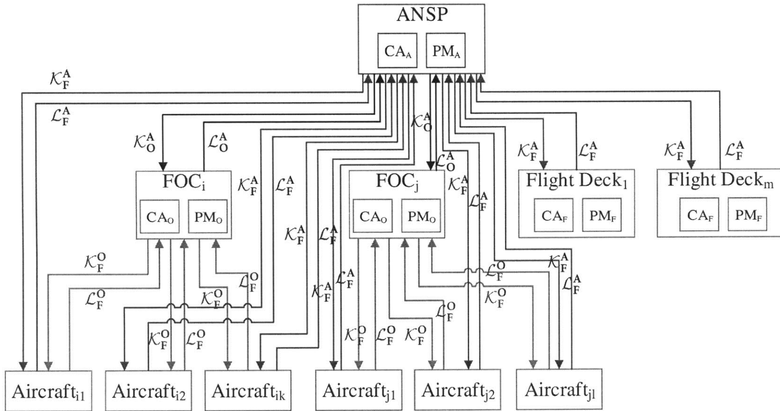
Figure 27: Nominal TBO Control Model—Trajectory Negotiation
