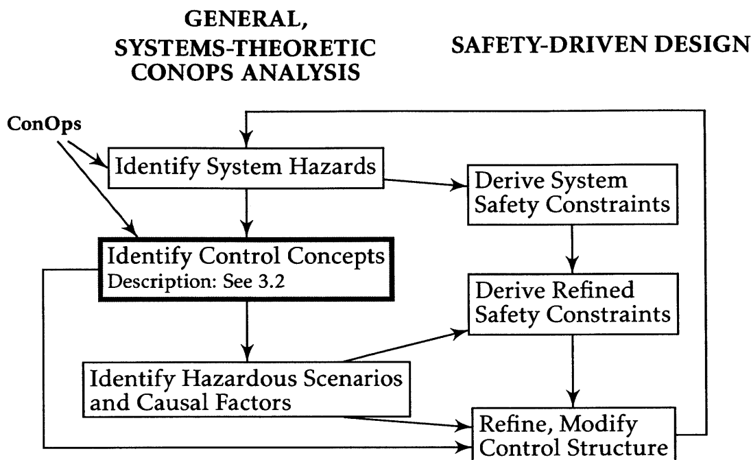
Figure 17: Methodology—Identifying Control Concepts
