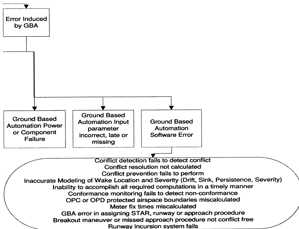
Figure 31: Software in Fault Tree Analysis [JPDO, 2012]
