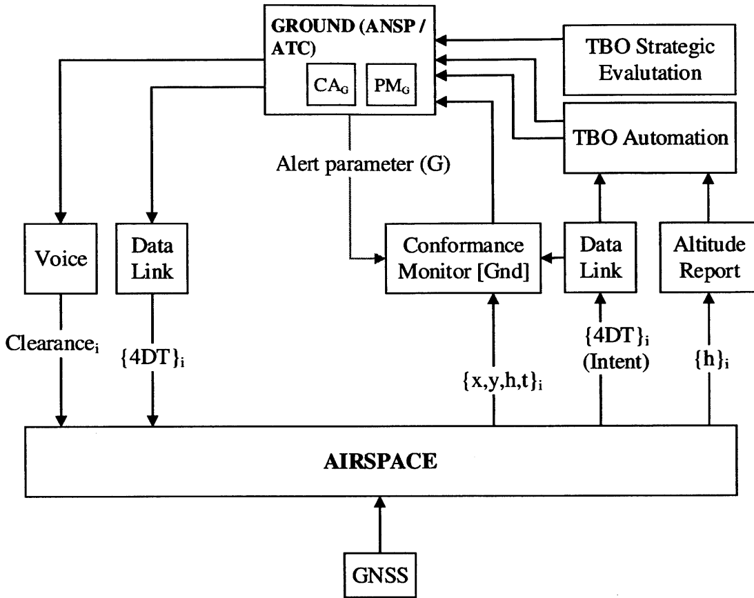
Figure 23: ANSP (Ground) Control Loops
