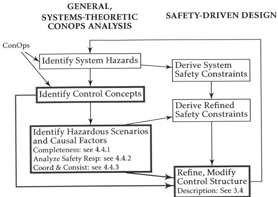
Figure 26: Methodology—Refine Safety Constraints
