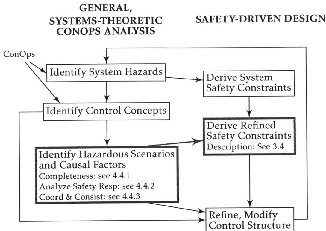
Figure 25: Methodology—Refine Safety Constraints
