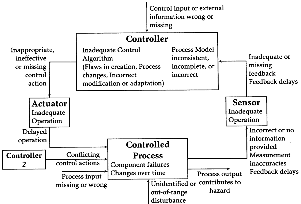
Figure 6: STPA Control Loop with Causal Factors
