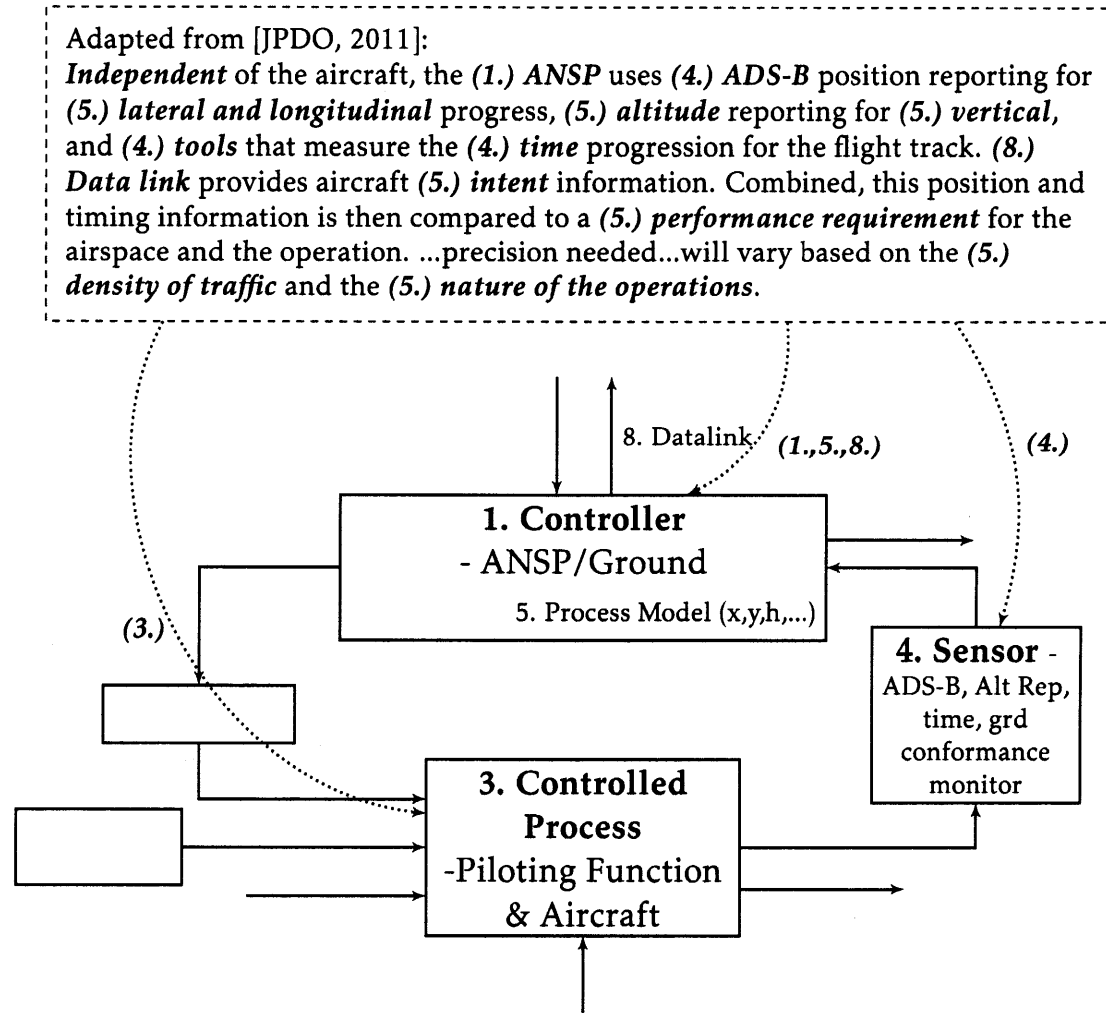
Figure 19: Graphical Control Model of Ground Conformance Monitor
