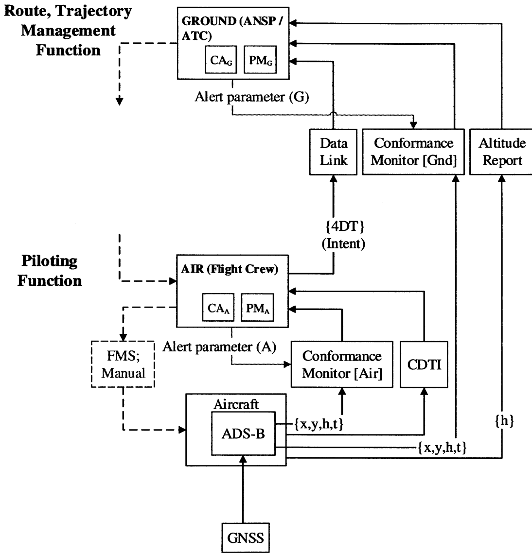
Figure 21: TBO Conformance Monitoring Control Structure
