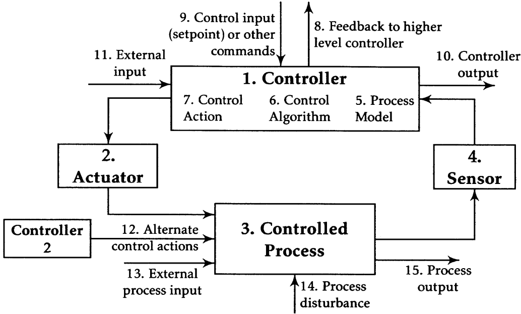
Figure 11: Control Loop with generic entities
