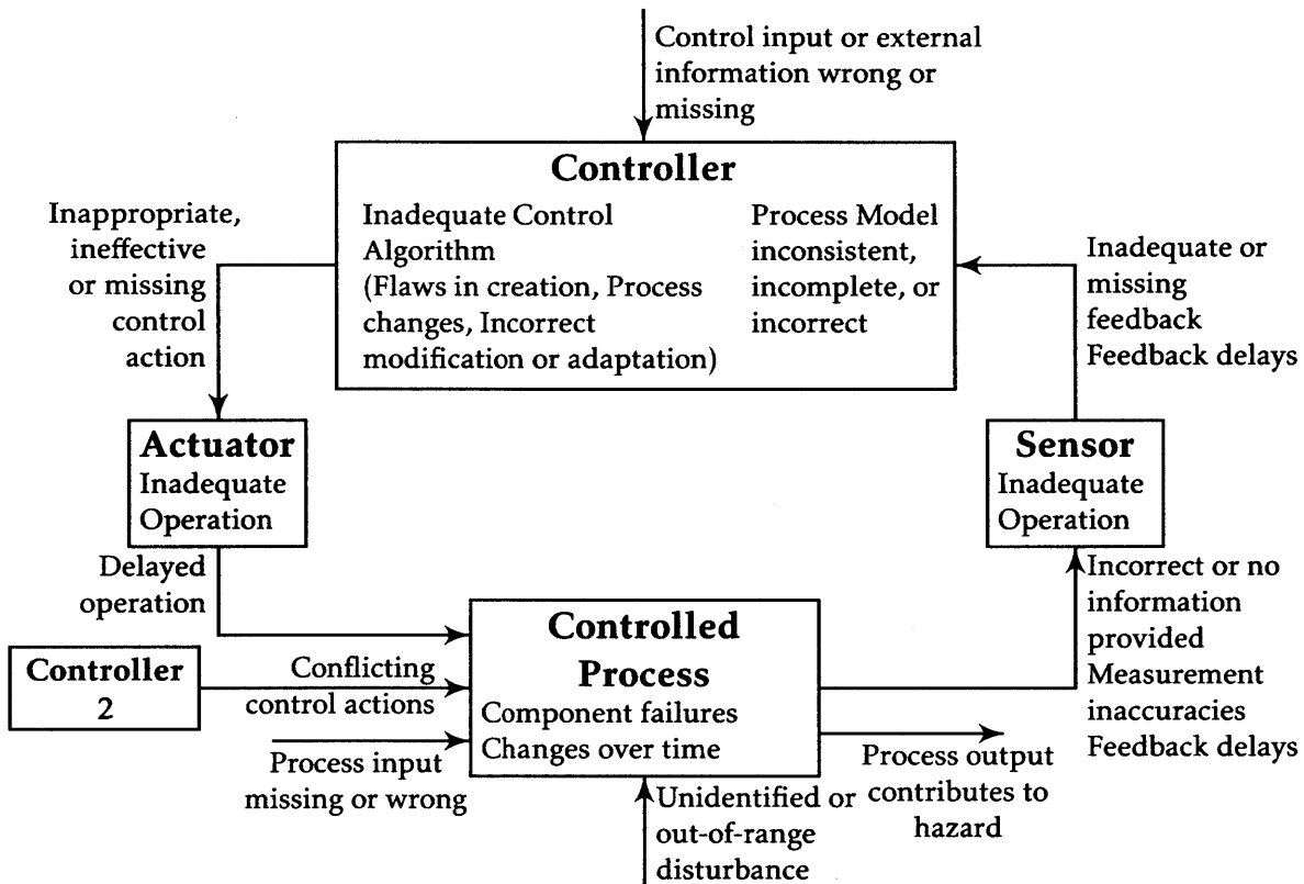
Figure 10: STPA Control Loop with Causal Factors
