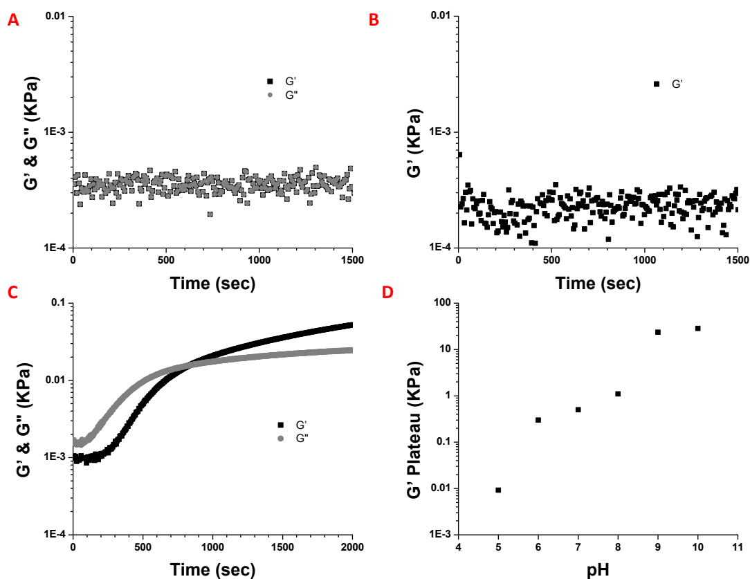
Figure 5.5 Sodium periodate mechanism: A) Elastic and viscous modulus of 70 MOEP-20% methacrylated polymer solution with 20 mM \text{NaIO}_4 , at pH 9 37° C. B) Elastic modulus of nonmethacrylated polyamine at pH 9, 37° C. C) Elastic and viscous modulus of nonmethacrylated polyamine at pH 9, with 20 mM \text{NaIO}_4 37° C. D) Elastic modulus plateau of 5% methacrylated polyamine at varied pH's, with 20 mM \text{NaIO}_4 , at 37°C.
