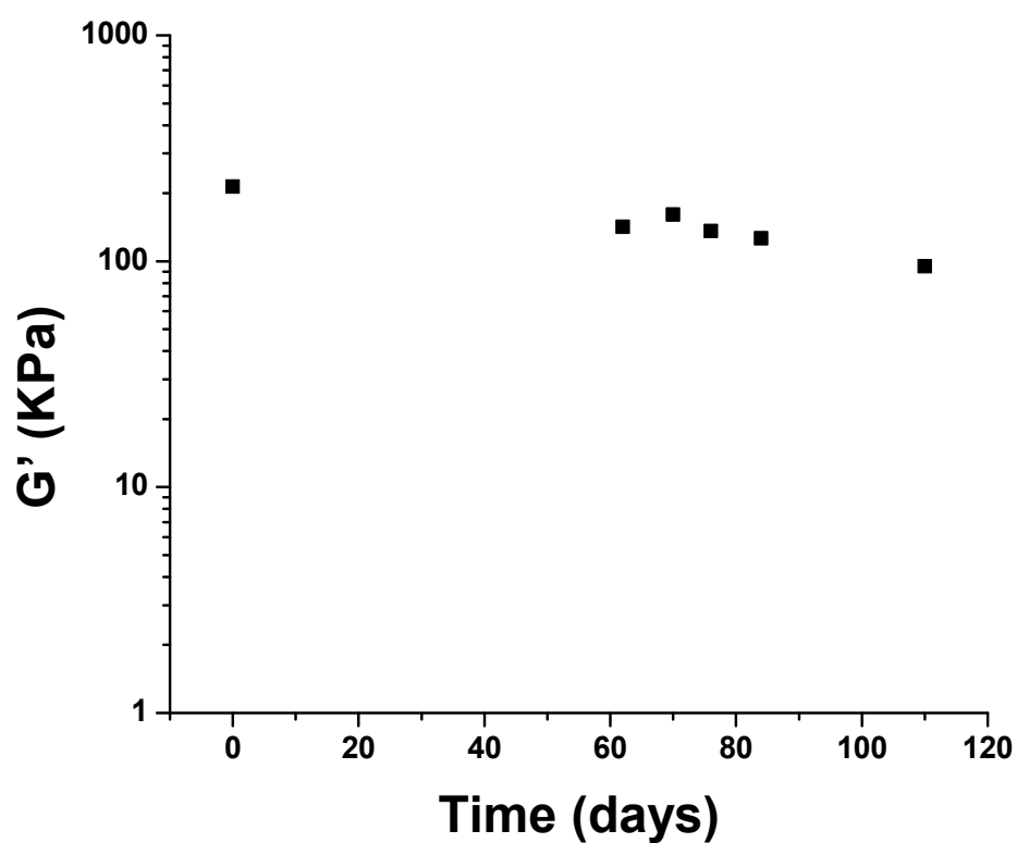
Figure 5.9 Stability study of complex coacervate adhesive sent for pig animal studies, made of 70 MOEP-20% methacrylation on the polyphosphate polymer and 5% methacrylation on the polyamine polymer, 10 wt% PEG-dMA within the coacervate, pH 7.2, with 35 mM \text{NaIO}_4 concentrations at 37°C. Showing plateau elastic modulus of samples that are chemically cured adhesive over a time period.
