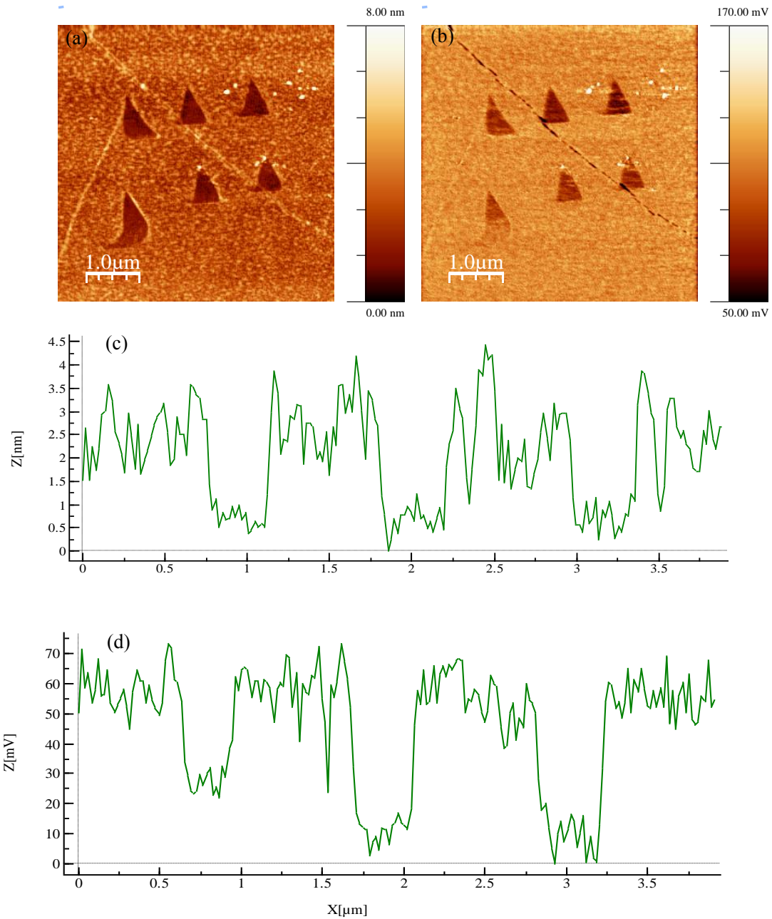
Fig. 4.7: AFM topography (a) and friction (b) images of rGF patterns. The patterns were created at a constant tip speed of 0.2 \mu\text{m/s} , a constant heater temperature of 950 \text{ }^\circ\text{C} and an increasing force setpoint from 0.2 \text{ V} to 1.7 \text{ V} with a step of 0.3 \text{ V} (the bottom left has the lowest setpoint and the top right has the highest setpoint). (c) and (d) are the cross sections of (a) and (b).
