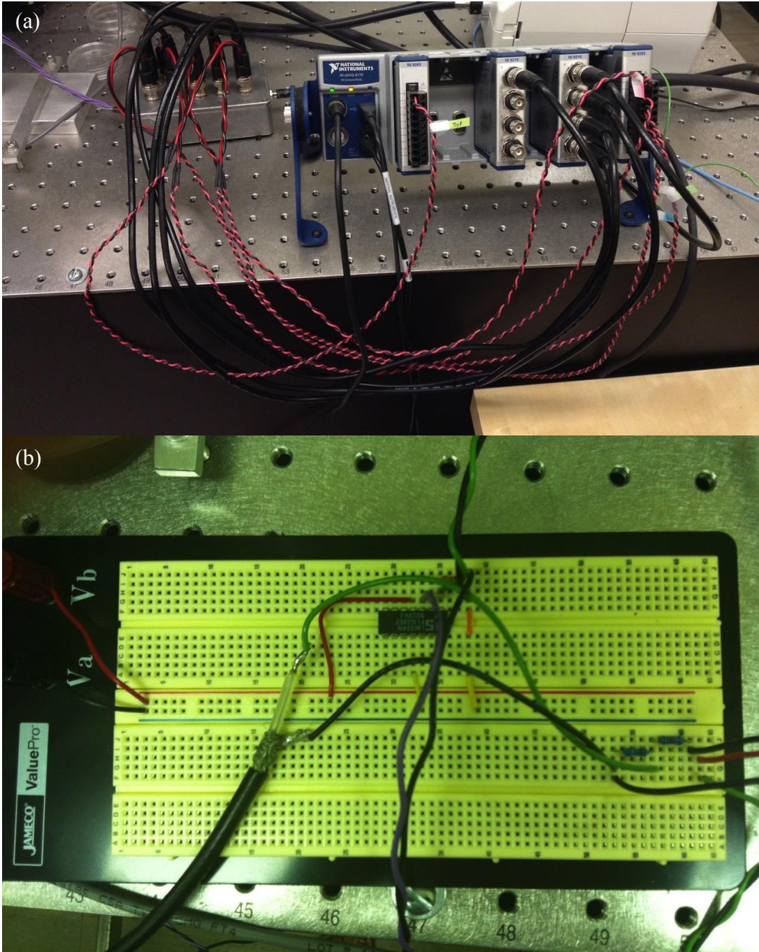
Fig. 3.8: Connection between the DAQ and array PCB. (a) The DAQ is connected to a shielding box, containing five identical circuits. The purple wires connect the shielding box to the array PCB. (b) A demonstration of just one circuit inside the shielding box. The circuit includes an operational amplifier chip and two 1 kOhm resistors.
