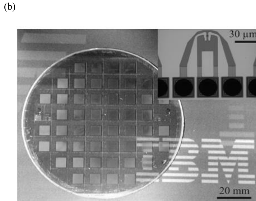
Fig. 1.3: Millipede cantilever array. (a) The millipede concept. (b) Glass wafer of cantilever arrays. Each square contains 4096 cantilevers. The inset shows the cantilever structure bonded on the glass wafer [49, 50].
