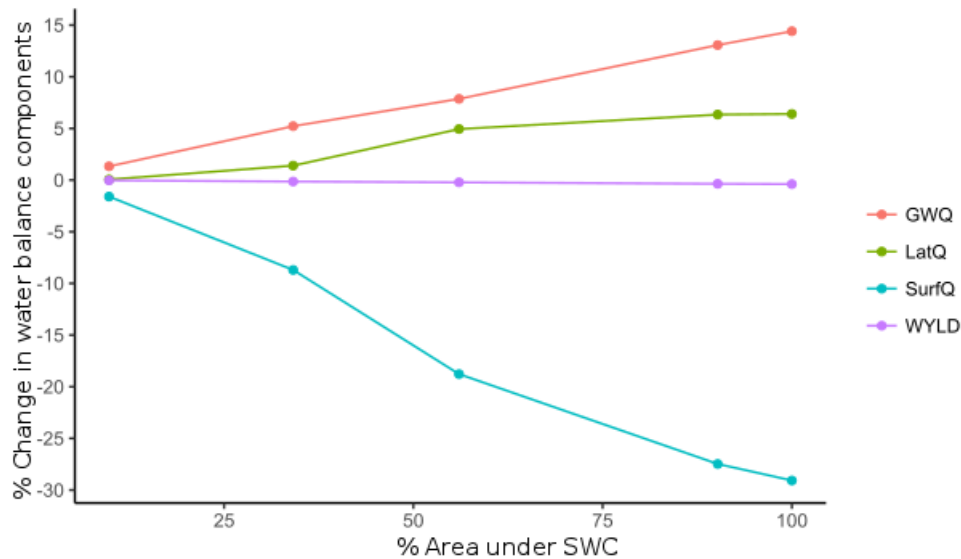
Figure 4.3.2: Effect of area under SWC on percentage change of water balance components (SurfQ = surface runoff, LatQ = lateral flow, GWQ = groundwater flow, WYLD = water yield)
