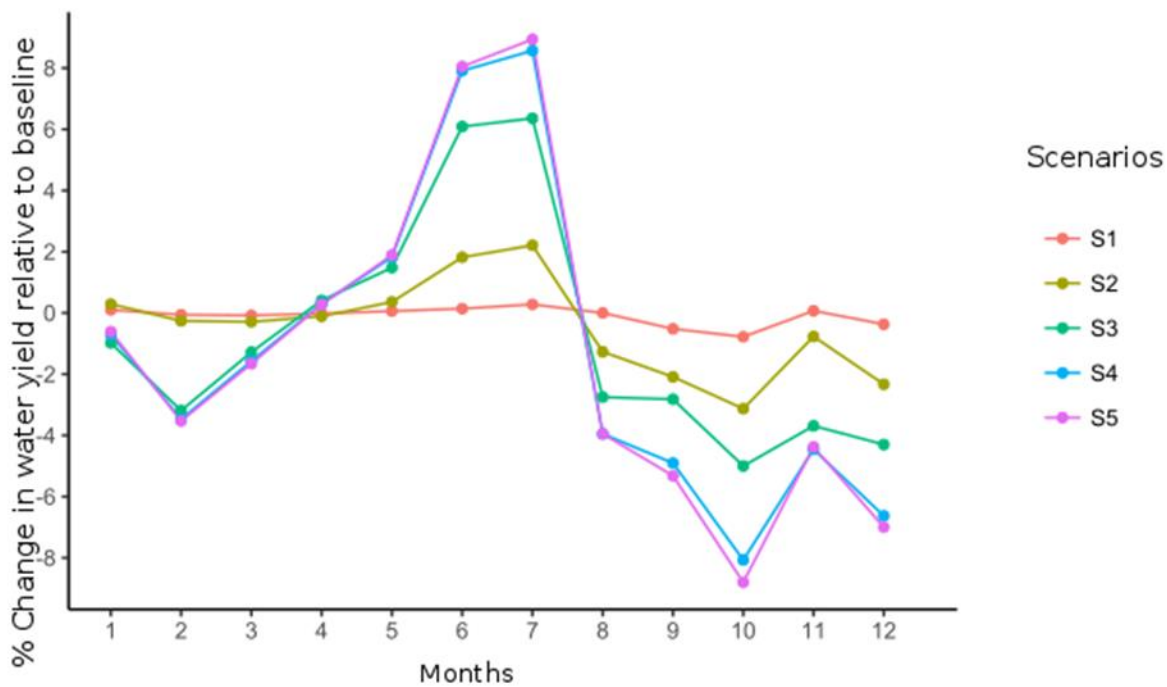
Figure 4.3.3: Seasonal variations in percentage change of water yield under SWC scenarios (8 years monthly averages, from 2007 - 2014). S1 = Contour farming, S2 = Fanya juu terracing, S3 = Bench terracing, S4 = Fanya juu + Bench terracing, S5 = Contour farming+ Fanya juu terracing + Bench terracing.
