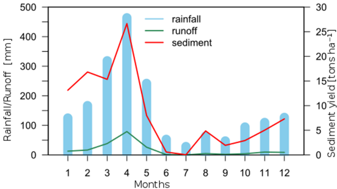
Figure 4.2.5: Catchment mean monthly rainfall, mean monthly surface runoff and mean monthly sediment yield (8 years monthly average for 2007-2014 period)
