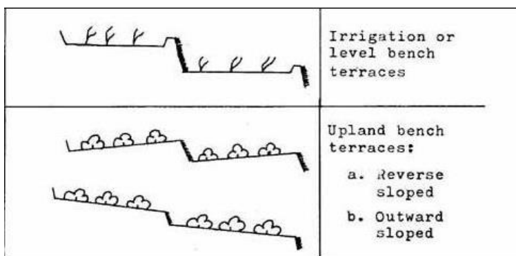
Figure 2. 5: Cross sectional view of bench terrace types (Sheng, 2000)
