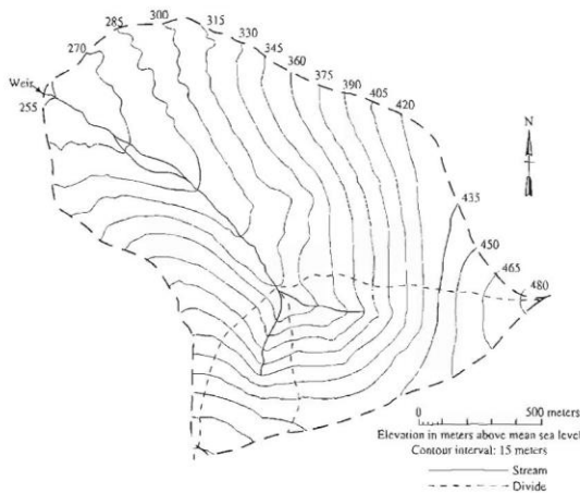
Figure 2.1: Watershed delineation on a topographic map (Dingman, 2002)
